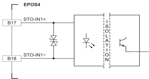
Figure 9-176 Safe Torque Off (STO) | STO-IN1 circuit (analogously valid for STO-IN2)
