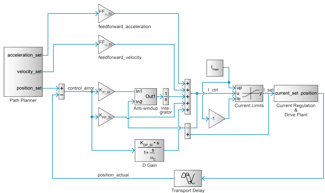
Figure 2-9 Controller architecture | Example 1: Position control with feedforward
