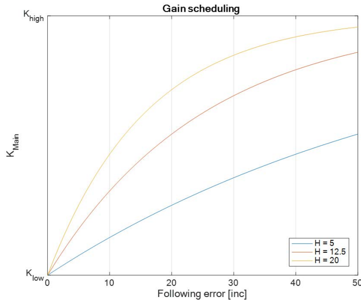
Figure 10-181 Dual loop control | Gain scheduling function for different values of main loop gain scheduling weight
