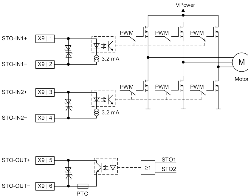
Figure 9-174 Safe Torque Off (STO) | Functional diagram
