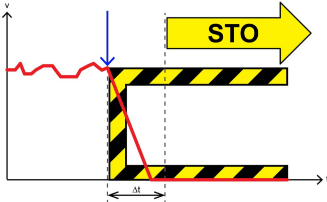
Figure 9-173 Safe Torque Off (STO) | Working principle
