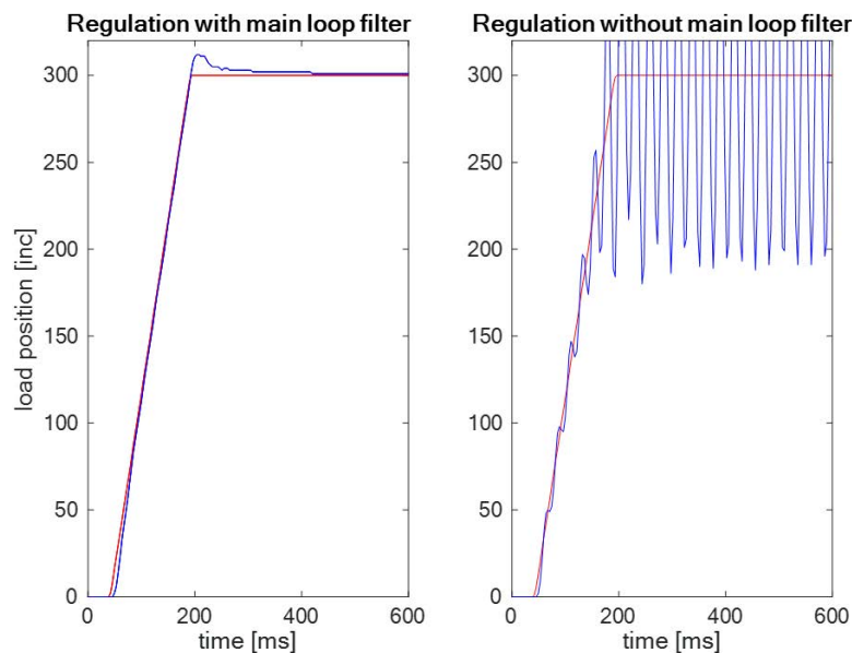
Figure 10-190 Dual loop control | Use case 2: Control performance with/without main loop filter
