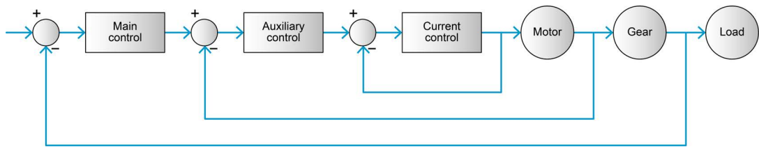
Figure 10-179 Dual loop control | Control structure
