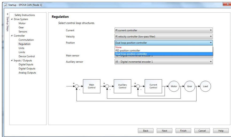
Figure 10-182 Dual loop control | Configuration
