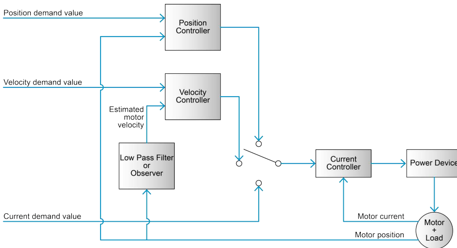
Figure 2-2 Controller architecture | Overview (simplified)
