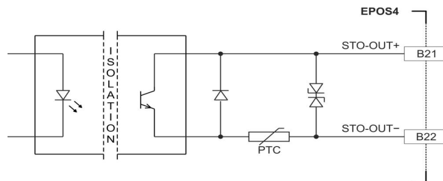
Figure 9-178 Safe Torque Off (STO) | STO-OUT circuit
