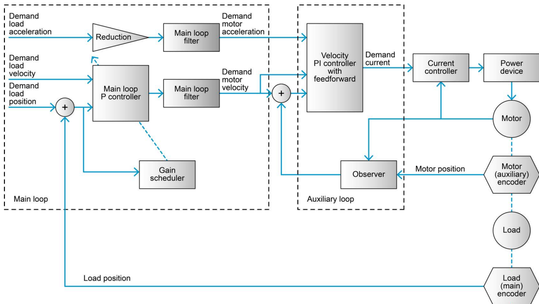
Figure 10-180 Dual loop control | Control structure in detail
