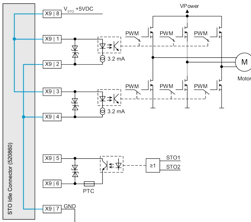
Figure 9-175 Safe Torque Off (STO) | STO Idle Connector
