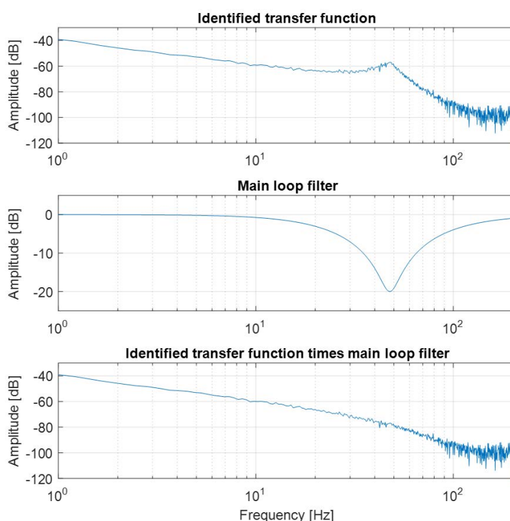
Figure 10-188 Dual loop control | Use case 2: Comparison of Bode plots
