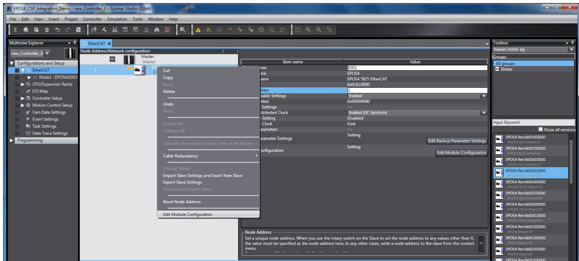
Figure 6-102 EtherCAT integration – OMRON Sysmac NJ | Slave parameters
