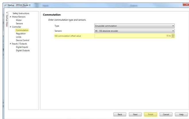
Figure 8-134 Adjustment of SSI commutation offset value | Set SSI commutation offset value
