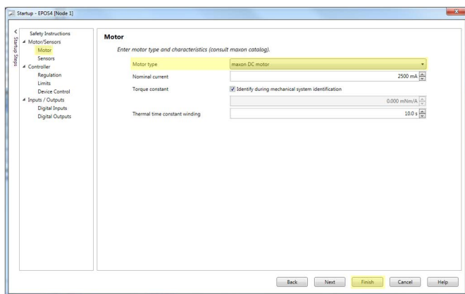
Figure 8-128 Adjustment of SSI commutation offset value | Select motor type maxon DC motor
