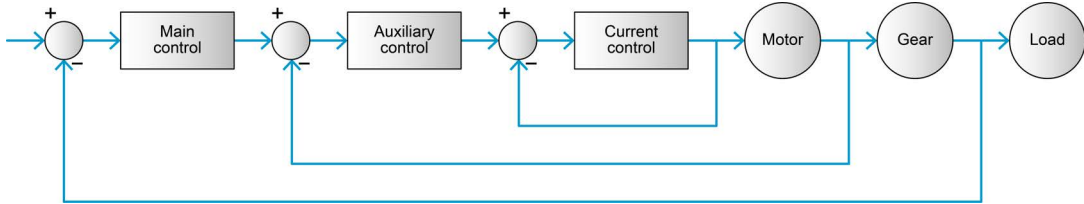
Figure 10-142 Dual loop control | Control structure
