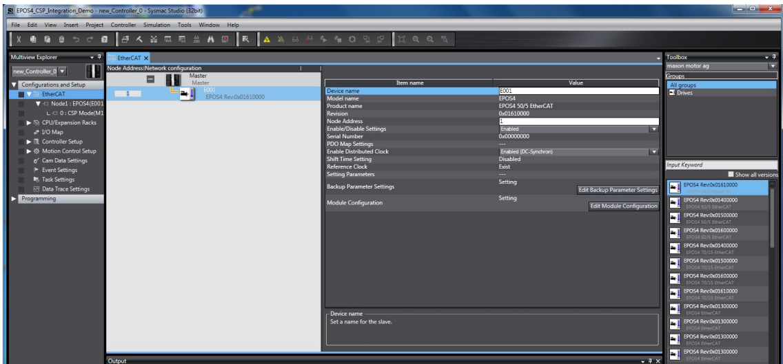
Figure 6-106 EtherCAT integration – OMRON Sysmac NJ | Set EtherCAT node address
