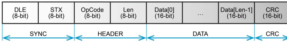
Figure 3-22 maxon serial protocol V1 vs. V2 | maxon serial V2 protocol – Frame structure
