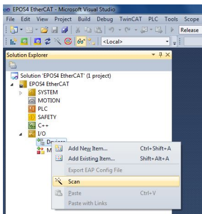
Figure 6-64 EtherCAT integration – Beckhoff TwinCAT | Scan devices
