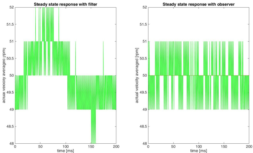
Figure 2-15 Controller architecture | Case 1: Comparison of velocity steady states
