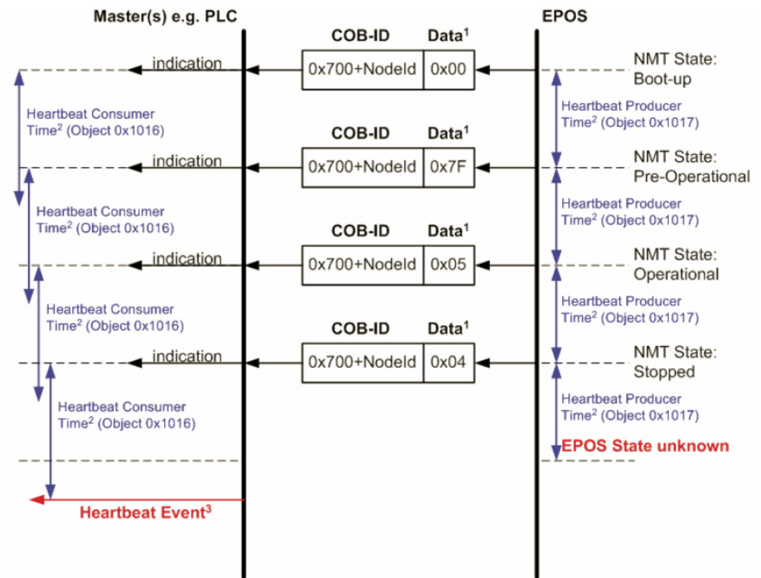
Figure 5-45 CANopen basic information | Heartbeat protocol – Timing diagram
