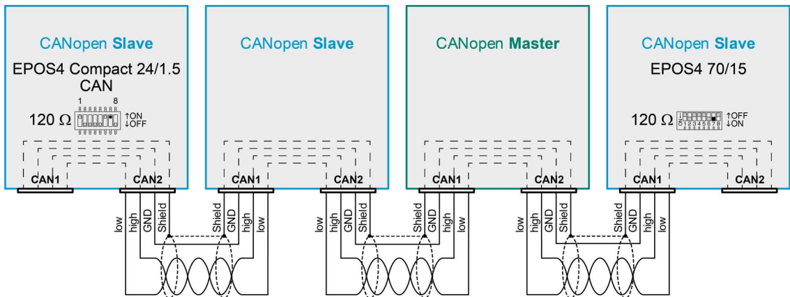
Figure 5-29 CANopen basic information | Topology with internal bus termination (example)
