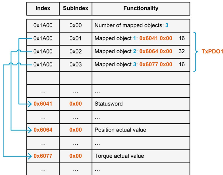
Figure 5-41 CANopen basic information | PDO mapping example
