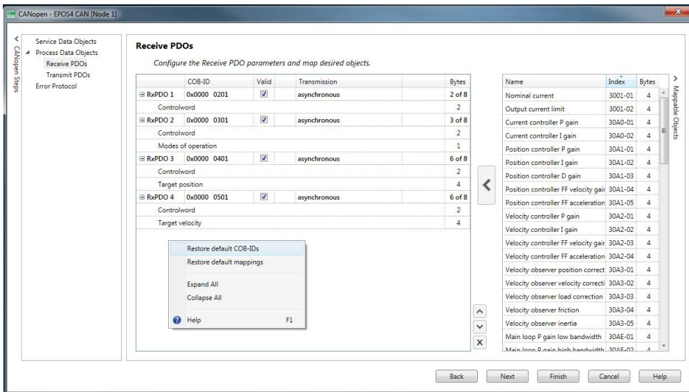
Figure 5-43 CANopen basic information | Receive PDOs: Restore default COB-IDs
