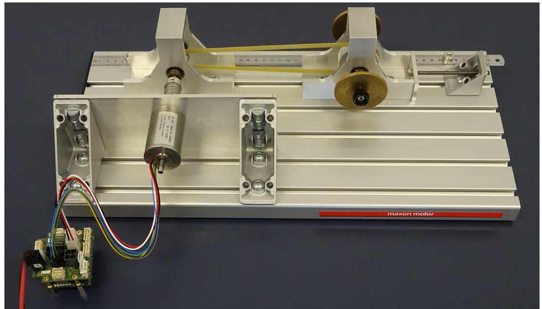
Figure 2-16 Controller architecture | Case 2: Belt drive system
