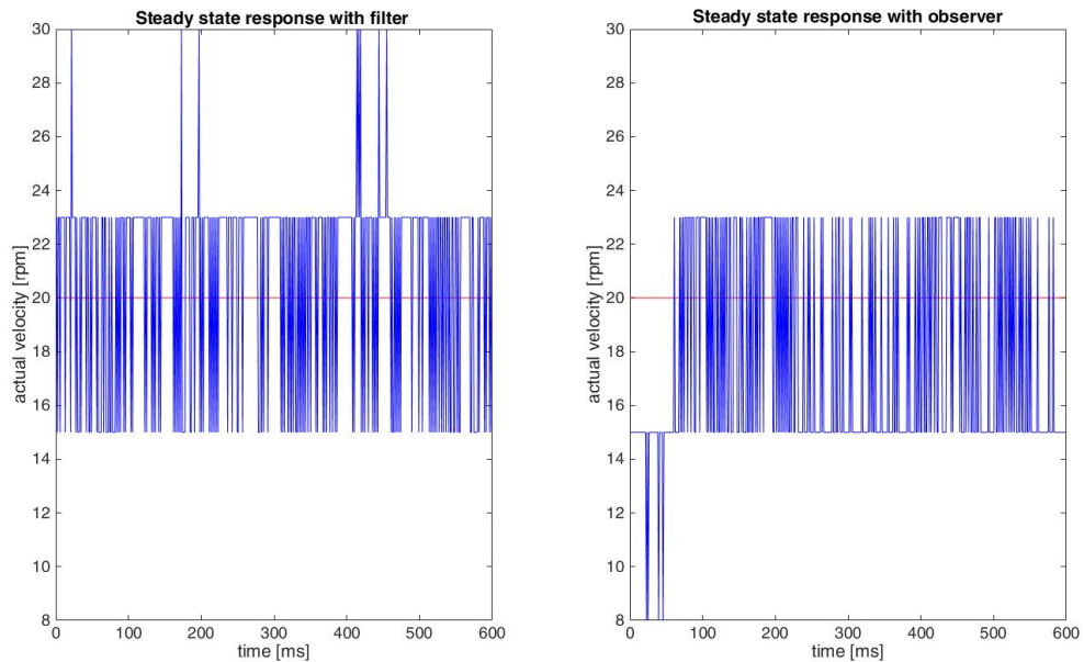
Figure 2-19 Controller architecture | Case 3: Comparison of velocity steady states
