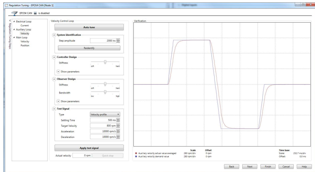
Figure 10-147 Dual loop control | Use case 1: Auxiliary loop tuning dialog box
