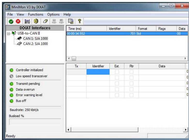
Figure 5-30 CANopen basic information | Example: Boot up message of node 1
