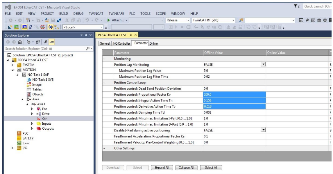
Figure 6-92 EtherCAT integration – Beckhoff TwinCAT | Configure position control parameters
