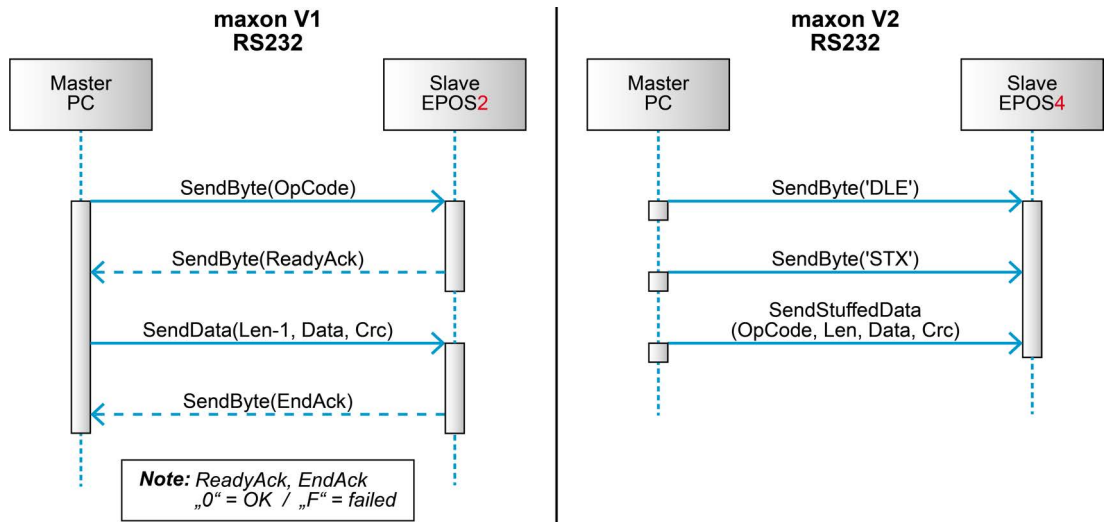
Figure 3-20 maxon serial protocol V1 vs. V2 | RS232 communication – Sending a data frame
