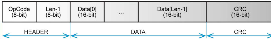
Figure 3-21 maxon serial protocol V1 vs. V2 | maxon serial V1 protocol – Frame structure
