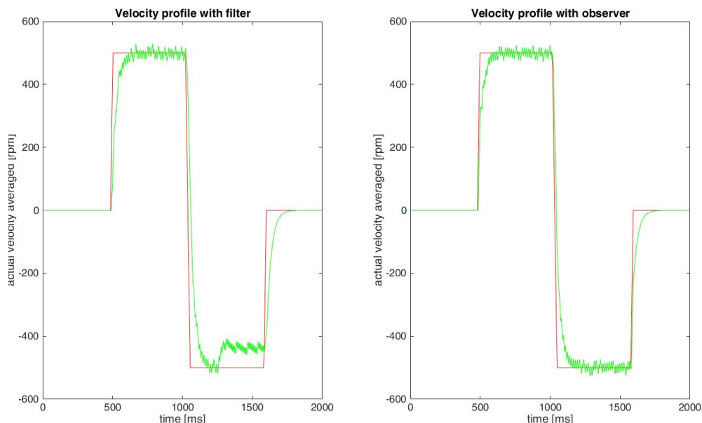
Figure 2-17 Controller architecture | Case 2: Comparison of velocity step responses
