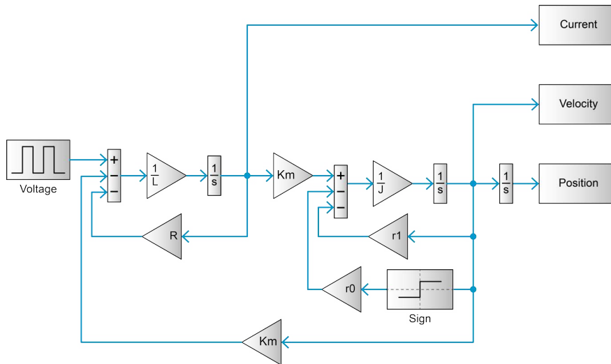
Figure 2-11 Controller architecture | Example 2: Model of the plant
