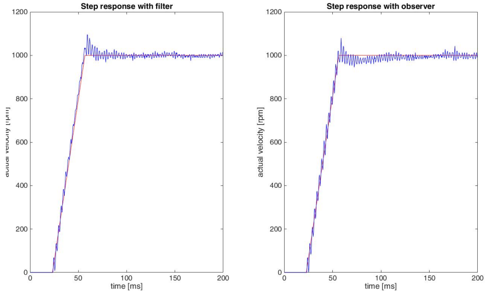
Figure 2-18 Controller architecture | Case 3: Comparison of velocity step responses
