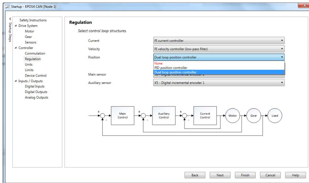
Figure 10-145 Dual loop control | Configuration
