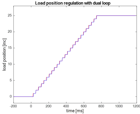
Figure 10-150 Dual loop control | Use case 1: Position control with dual loop controller
