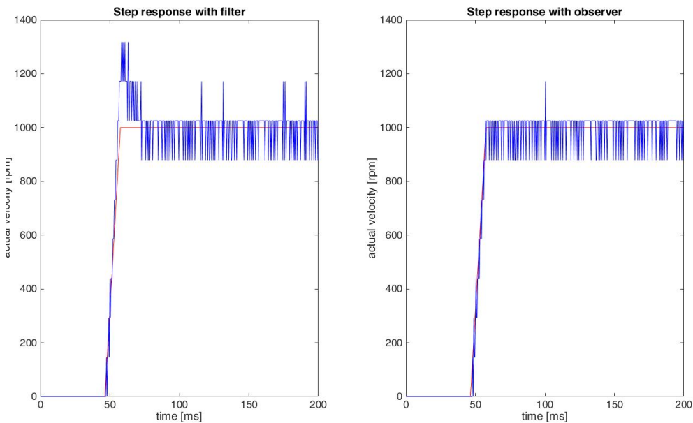
Figure 2-13 Controller architecture | Case 1: Comparison of velocity step responses
