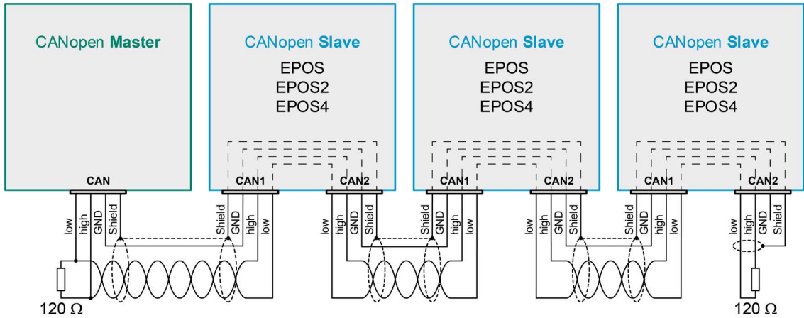
Figure 5-28 CANopen basic information | Topology with external bus termination (example)
