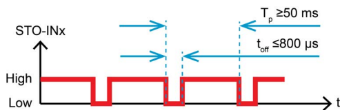
Figure 9-140 Safe Torque Off (STO) | Test pulses
