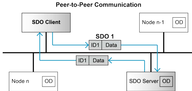
Figure 5-31 CANopen basic information | SDO communication
