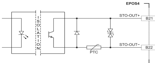
Figure 9-141 Safe Torque Off (STO) | STO-OUT circuit
