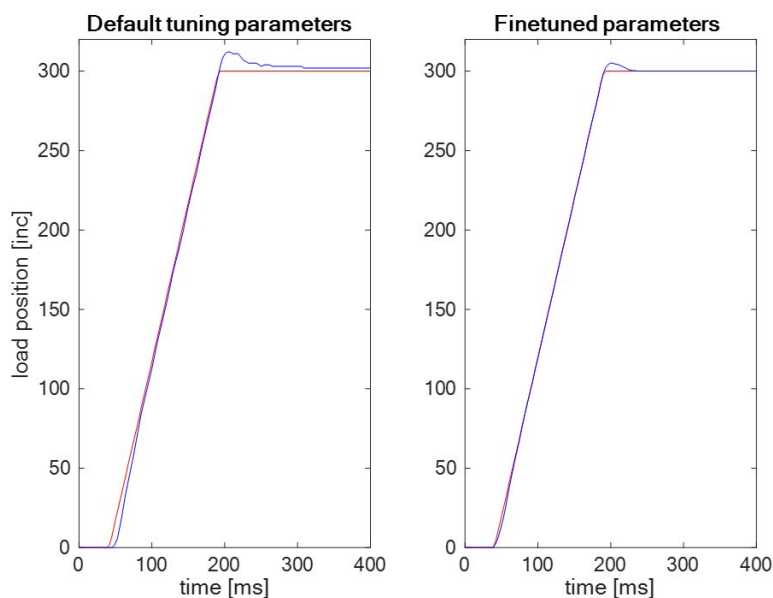
Figure 10-154 Dual loop control | Use case 2: Control performance with default/fine-tuned main loop parameters
