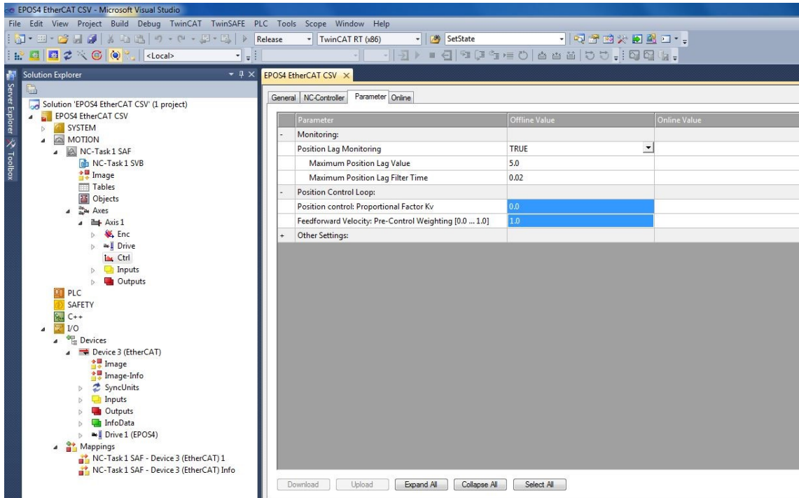
Figure 6-86 EtherCAT integration – Beckhoff TwinCAT | Set position control loop settings
