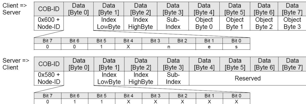
Figure 5-33 CANopen basic information | SDO upload protocol (expedited transfer) – Write
