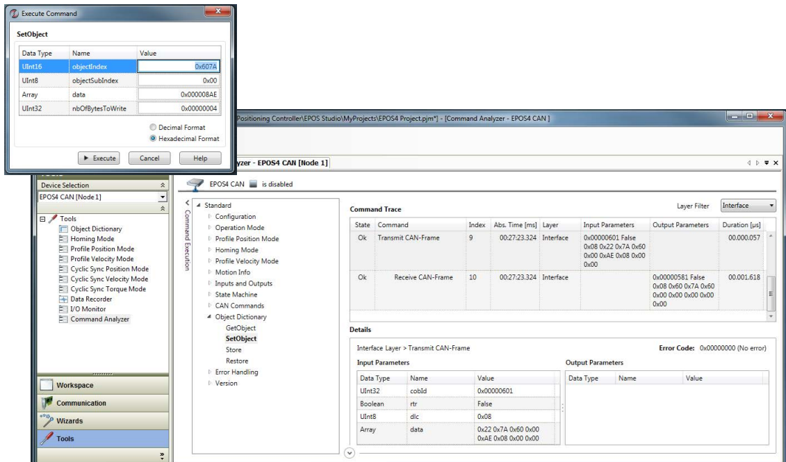
Figure 5-38 CANopen basic information | Command example – Write Object (= SetObject)
