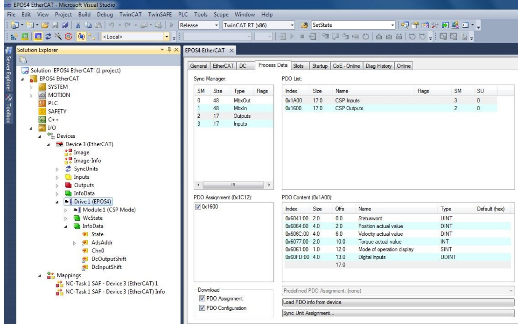
Figure 6-73 EtherCAT integration – Beckhoff TwinCAT | Display process data
