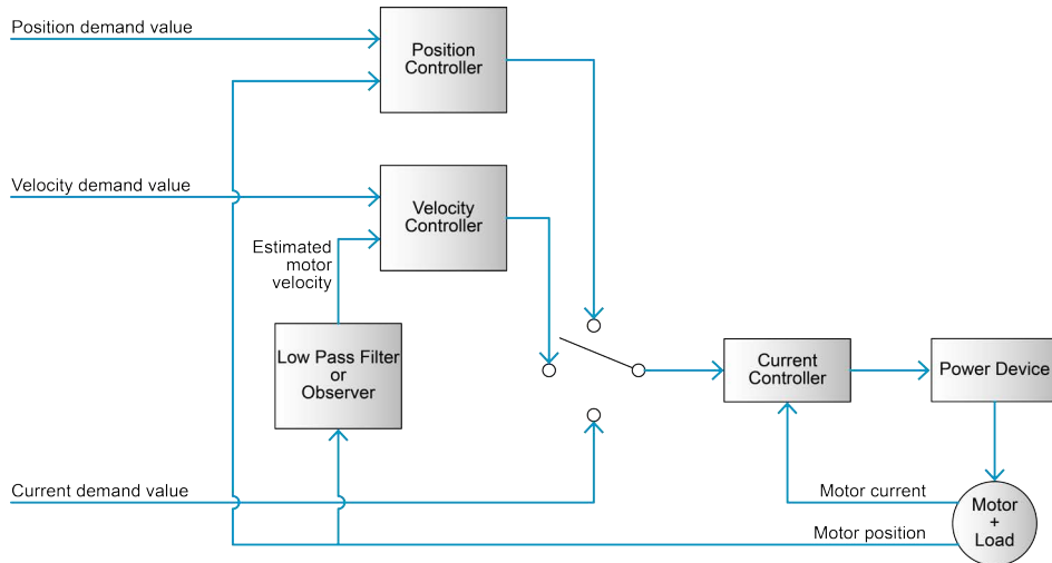
Figure 2-2 Controller architecture | Overview (simplified)
