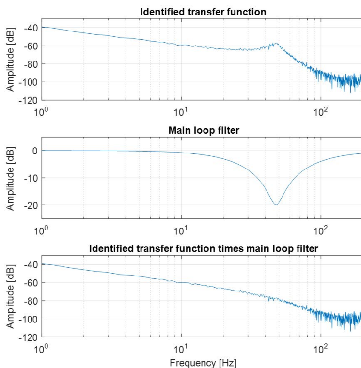
Figure 10-151 Dual loop control | Use case 2: Comparison of Bode plots
