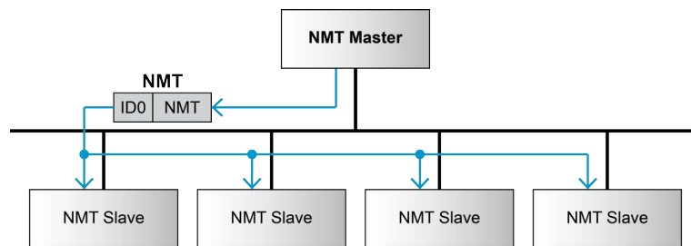
Figure 5-39 CANopen basic information | Network Management (NMT)
