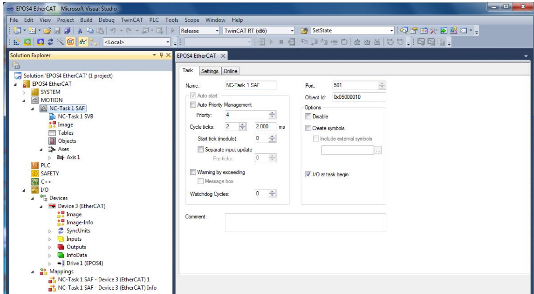
Figure 6-77 EtherCAT integration – Beckhoff TwinCAT | Set cycle ticks 1
