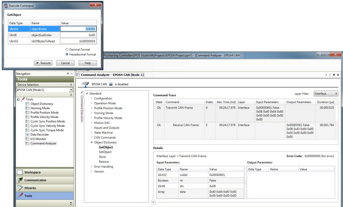
Figure 5-37 CANopen basic information | Command example – Read Object (= GetObject)
