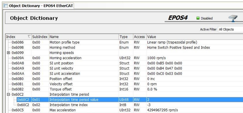
Figure 6-78 EtherCAT integration – Beckhoff TwinCAT | Set cycle ticks 2
