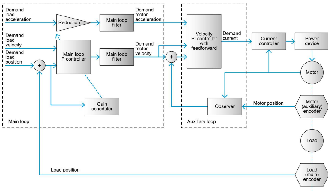
Figure 10-143 Dual loop control | Control structure in detail
