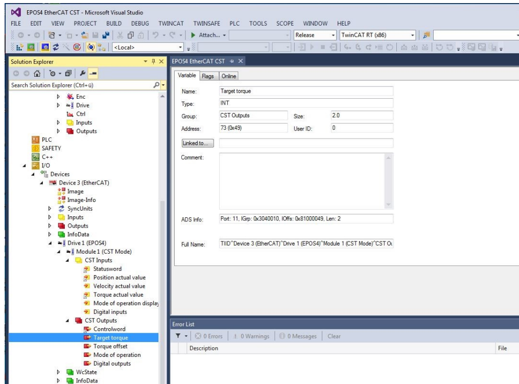
Figure 6-89 EtherCAT integration – Beckhoff TwinCAT | Set target torque
