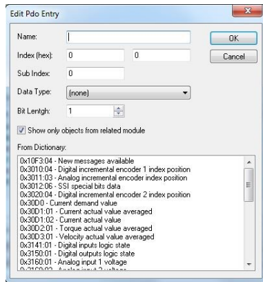
Figure 6-75 EtherCAT integration – Beckhoff TwinCAT | Edit PDO values
