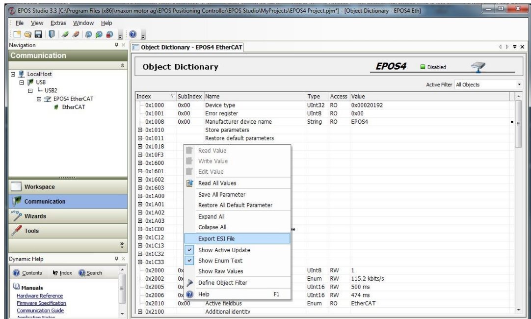
Figure 6-61 EtherCAT integration – Beckhoff TwinCAT | Export ESI file
