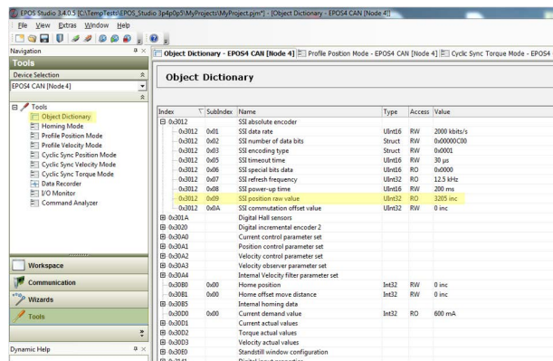
Figure 8-131 Adjustment of SSI commutation offset value | Read SSI position raw value
