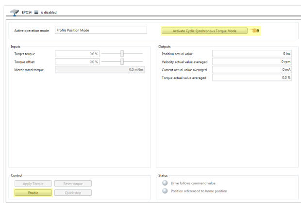
Figure 8-129 Adjustment of SSI commutation offset value | Activate CST
