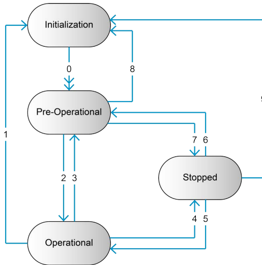
Figure 5-40 CANopen basic information | NMT slave state diagram
