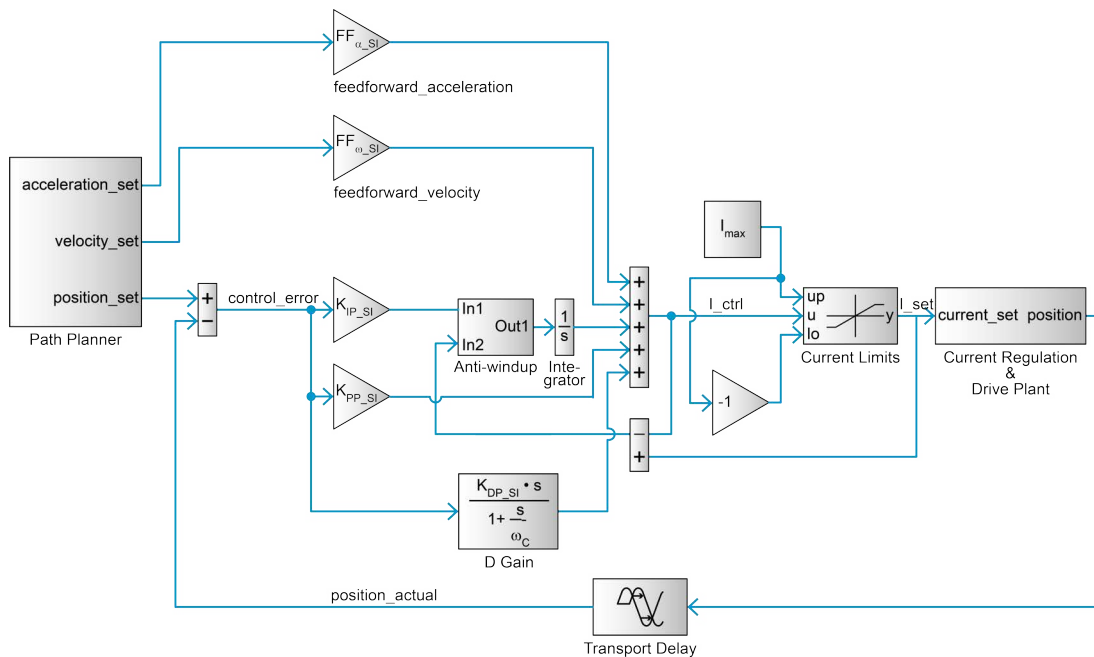
Figure 2-9 Controller architecture | Example 1: Position control with feedforward
