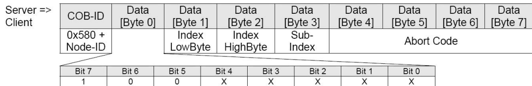
Figure 5-34 CANopen basic information | SDO upload protocol (expedited transfer) – Abort
