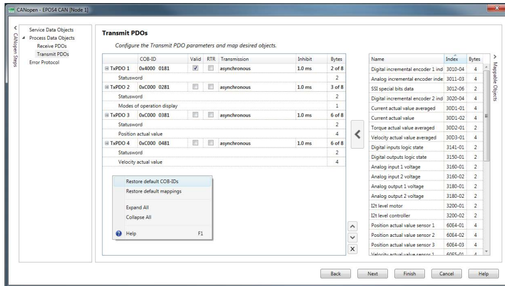
Figure 5-44 CANopen basic information | Transmit PDOs: Restore default COB-IDs
