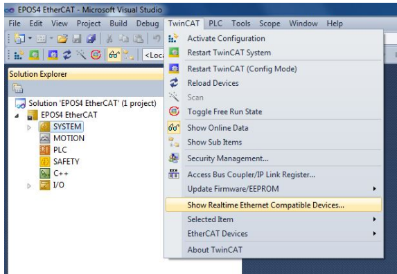
Figure 6-62 EtherCAT integration – Beckhoff TwinCAT | Create new project
