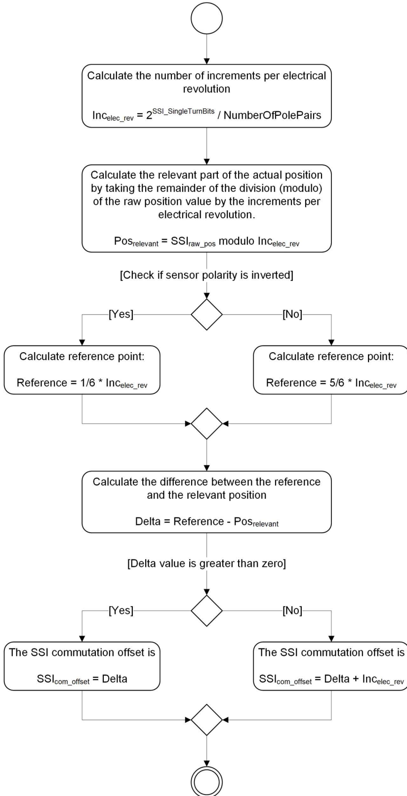
Figure 8-132 Adjustment of SSI commutation offset value | Determine SSI commutation offset value
