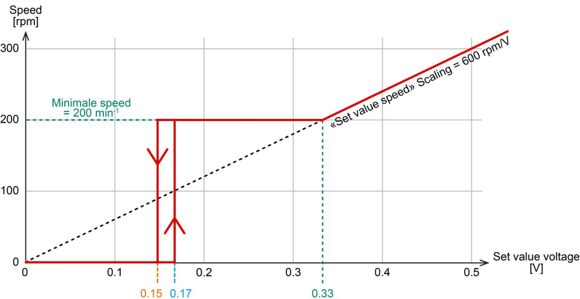
Figure 3-5 Input «Set value speed» – Switch on/switch off hysteresis (detail)
