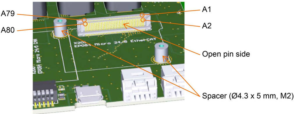
Figure 4-61 EPOS4 Micro 24/5 EtherCAT – Terminal/socket placement (example)
