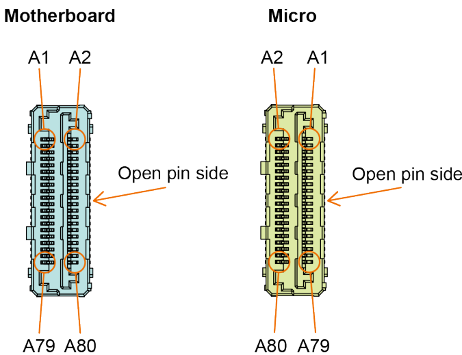
Figure 4-62 EPOS4 Micro 24/5 EtherCAT – Terminal/socket placement (mating)
