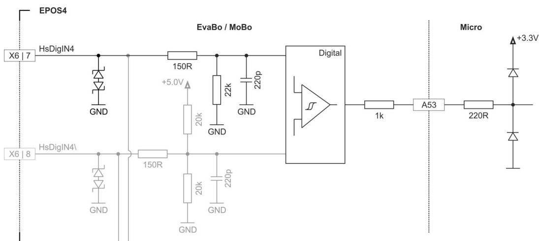
Figure 3-41 HsDigIN4 circuit "single-ended"
