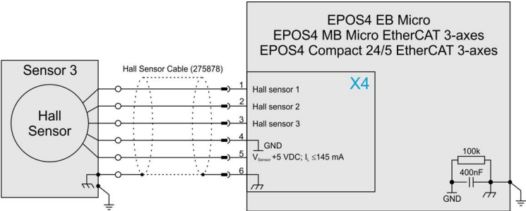
Figure 5-71 Hall sensors (Sensor 3)
