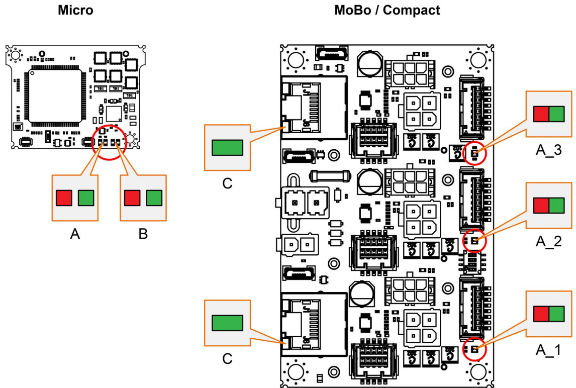
Figure 3-51 LEDs – Location
