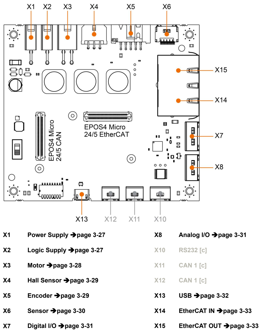
Figure 3-10 Connector Boards – Connectors
