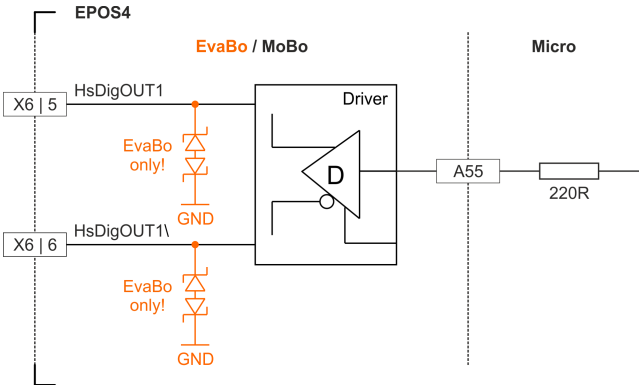
Figure 3-42 HsDigOUT1 output circuit
