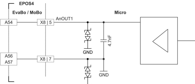
Figure 3-50 AnOUT1 circuit
