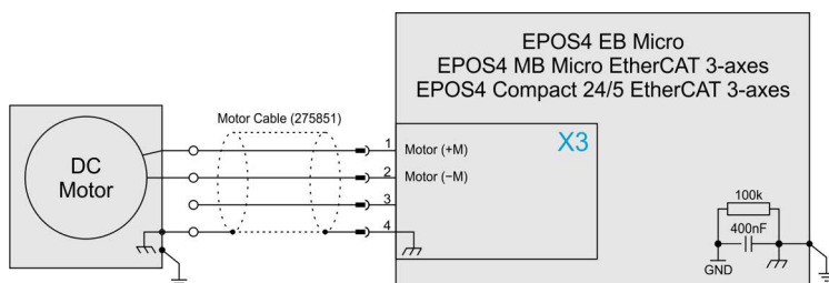
Figure 5-69 DC motor
