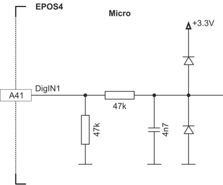
Figure 3-43 DigIN1 circuit (analogously valid for DigIN2...4) – Micro
