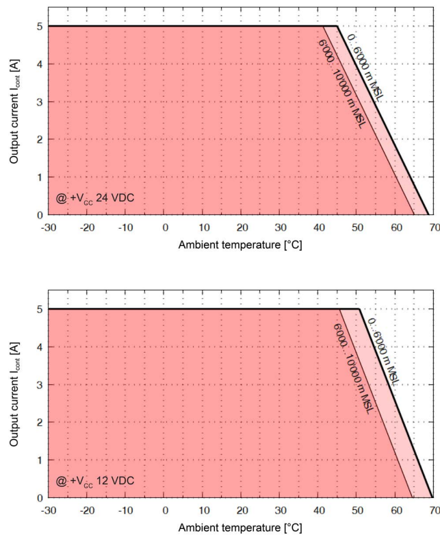
Figure 2-2 Derating of output current
