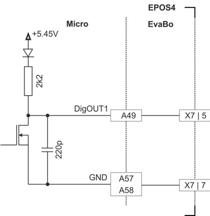
Figure 3-32 DigOUT1 circuit (analogously valid for DigOUT2)
