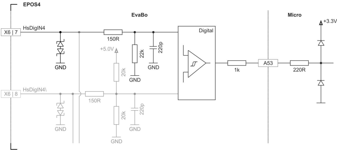
Figure 3-27 HsDigIN4 circuit "single-ended"
