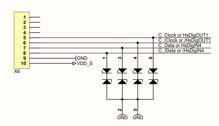
Figure 4-45 High-speed digital input/output and sensor protection circuitry
