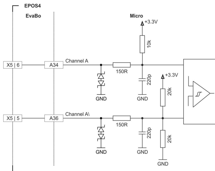
Figure 3-22 Encoder input circuit Ch A “differential” (analogously valid for Ch B &amp; Ch I)
