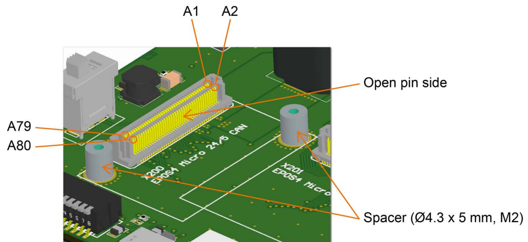
Figure 4-46 EPOS4 Micro 24/5 CAN – Terminal/socket placement (example)
