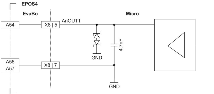
Figure 3-36 AnOUT1 circuit
