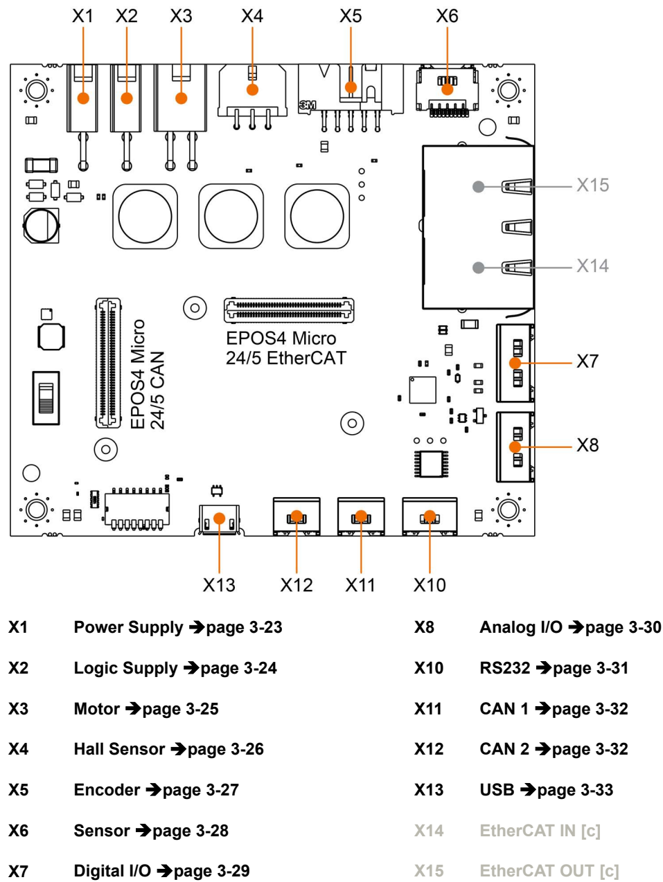
Figure 3-8 Connector Boards – Connectors
