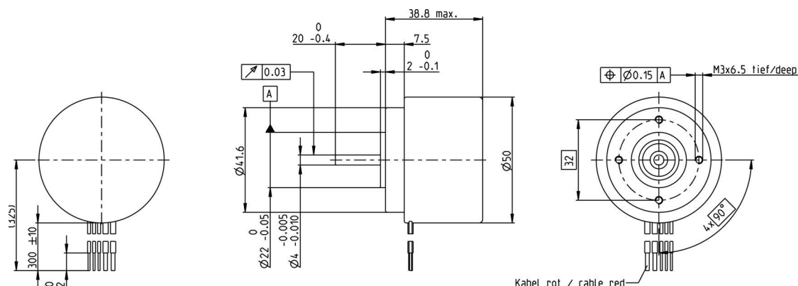
Figure 2-4 50 Watt version / IP40 – Dimensional drawing [mm]
