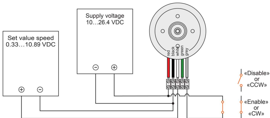
Figure 4-13 Speed set value with external power source and «Enable» or «Direction» with potential-free contact
