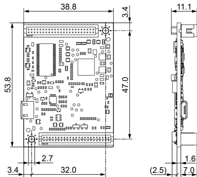
Figure 2-6 EPOS4 Module 50/5 – Dimensional drawing [mm]
