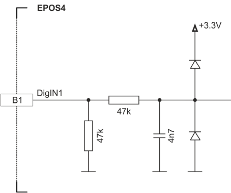
Figure 3-41 DigIN1 circuit (analogously valid for DigIN2...4) – Module
