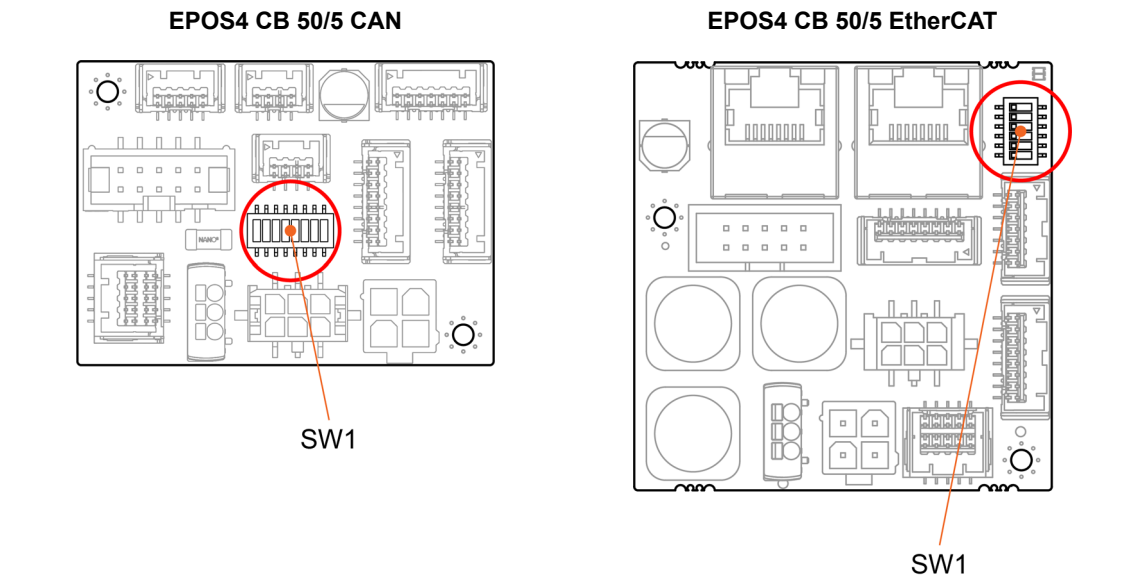
Figure 3-26 DIP switch SW1
