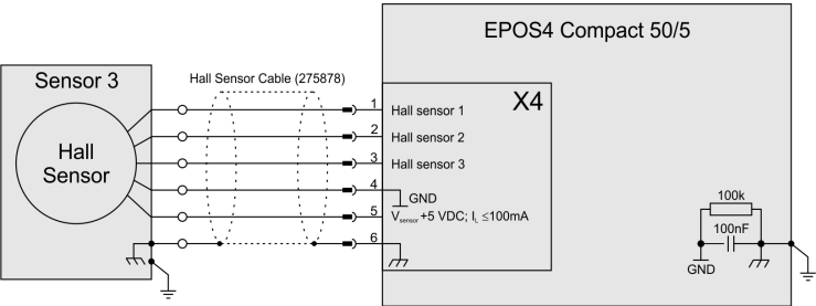
Figure 5-65 Hall sensors (Sensor 3)
