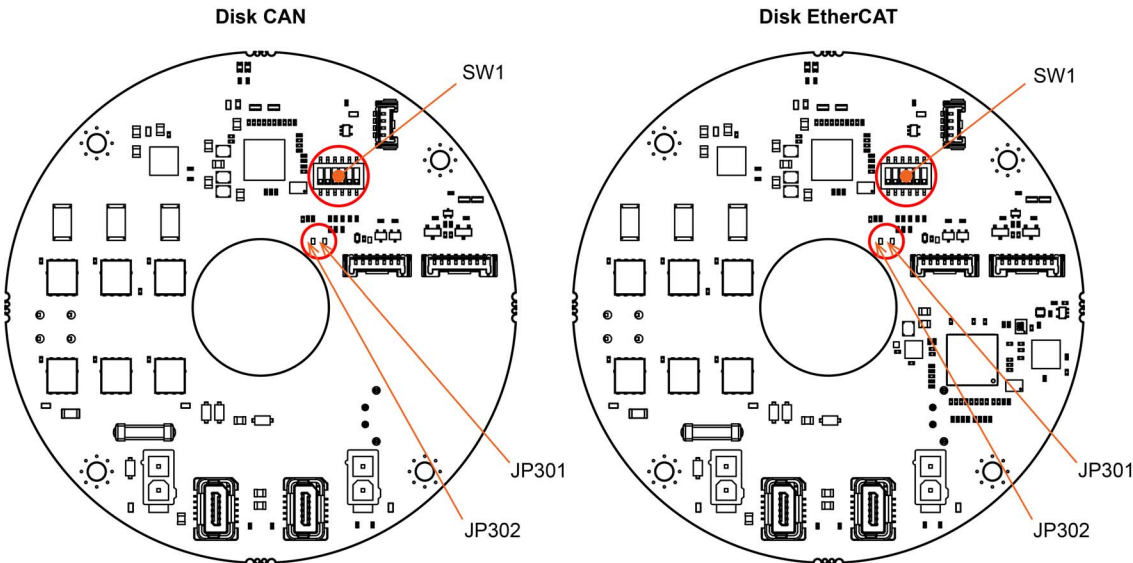
Figure 3-39 DIP switch SW1 and solder pads – Location
