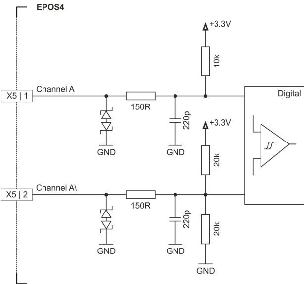
Figure 3-21 Digital incremental encoder input circuit Ch A “differential” (analogously valid for Ch B, Ch I, and X5/X6)
