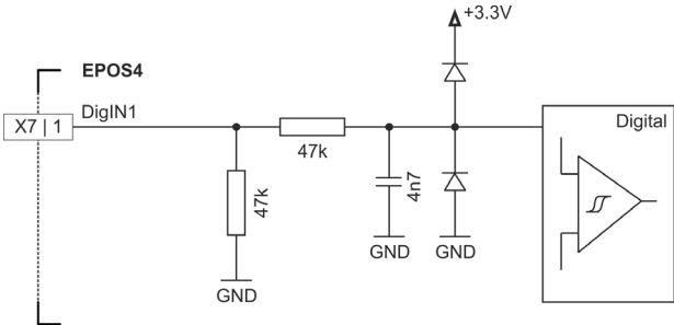
Figure 3-27 DigIN1 circuit (analogously valid for DigIN2...4 and X7a)
