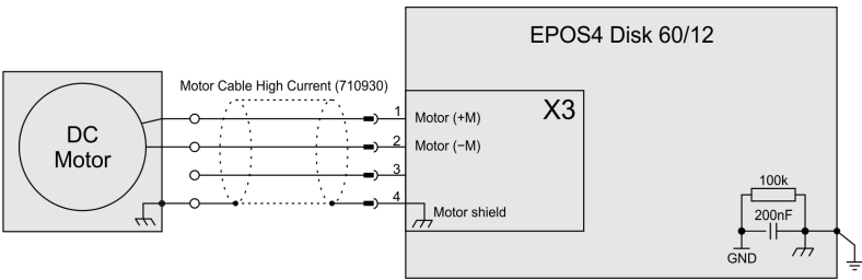
Figure 4-46 DC motor
