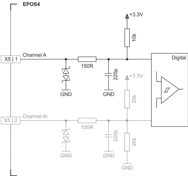
Figure 3-22 Digital incremental encoder input circuit Ch A “single-ended” (analogously valid for Ch B, Ch I, and X5/X6)
