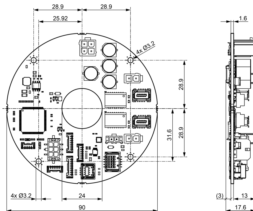
Figure 2-7 EPOS4 Disk 60/12 EtherCAT SSC (709862) – Dimensional drawing [mm]
