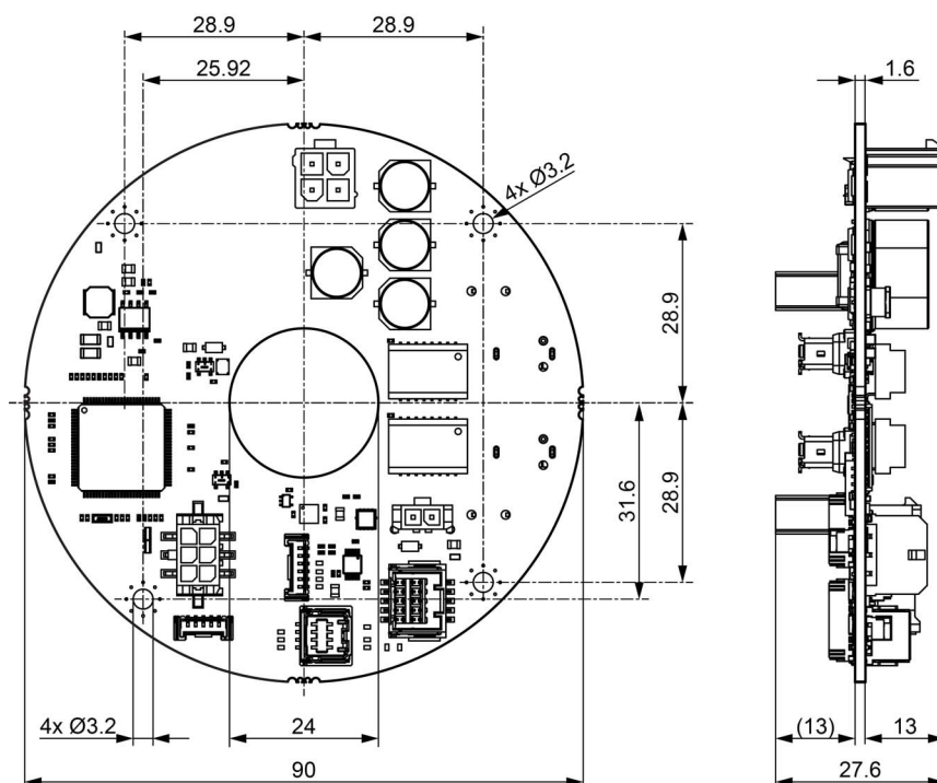
Figure 2-6 EPOS4 Disk 60/12 EtherCAT (688777) – Dimensional drawing [mm]
