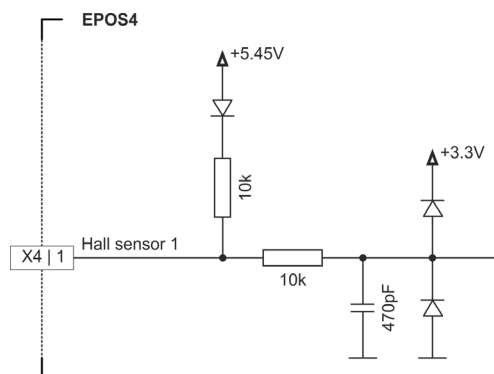
Figure 3-17 Hall sensor 1 input circuit (analogously valid for Hall sensors 2 &amp; 3 and X4a)
