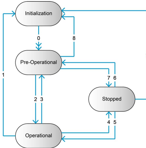
Figure 3-22 CAN communication – NMT slave states
