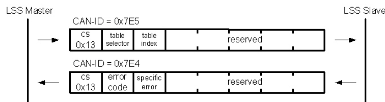
Figure 3-28 LSS – Configure Bit Timing Parameters
