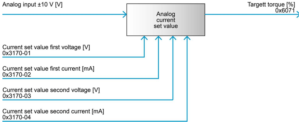
Figure 6-38 Analog input current set value properties – Setpoint function
