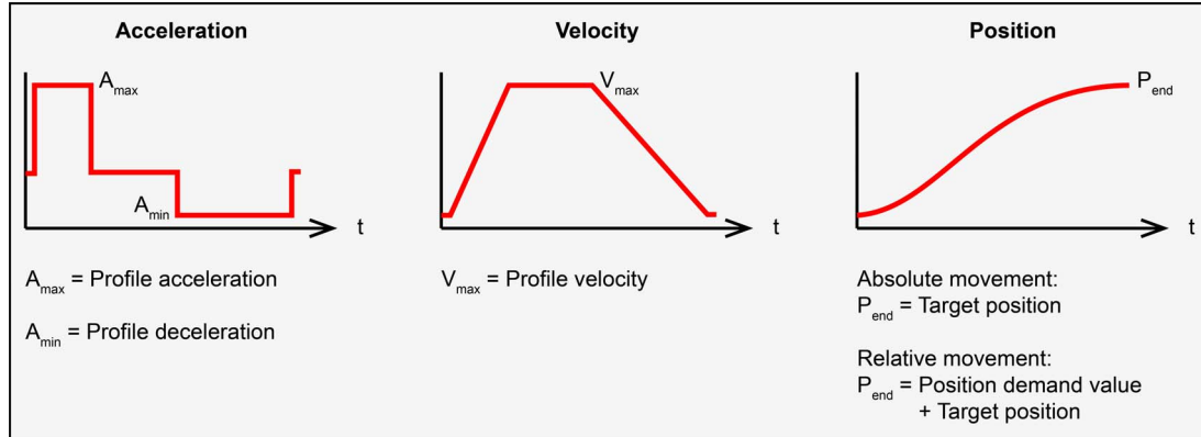
Figure 3-6 Profile position trajectory
