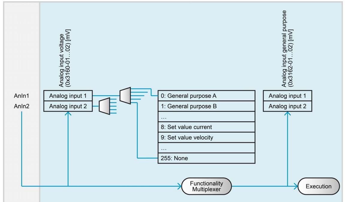
Figure 4-30 Analog input functionality
