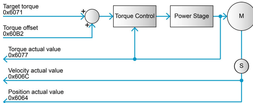
Figure 3-23 Cyclic Synchronous Torque Mode – Overview
