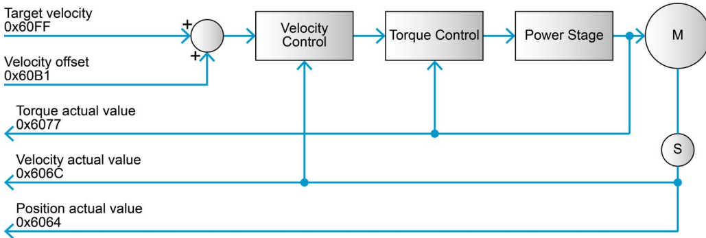
Figure 3-21 Cyclic Synchronous Velocity Mode – Overview
