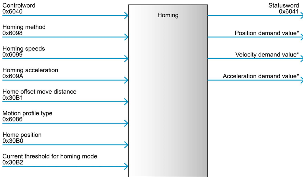
Figure 3-10 Homing Mode – Block diagram
