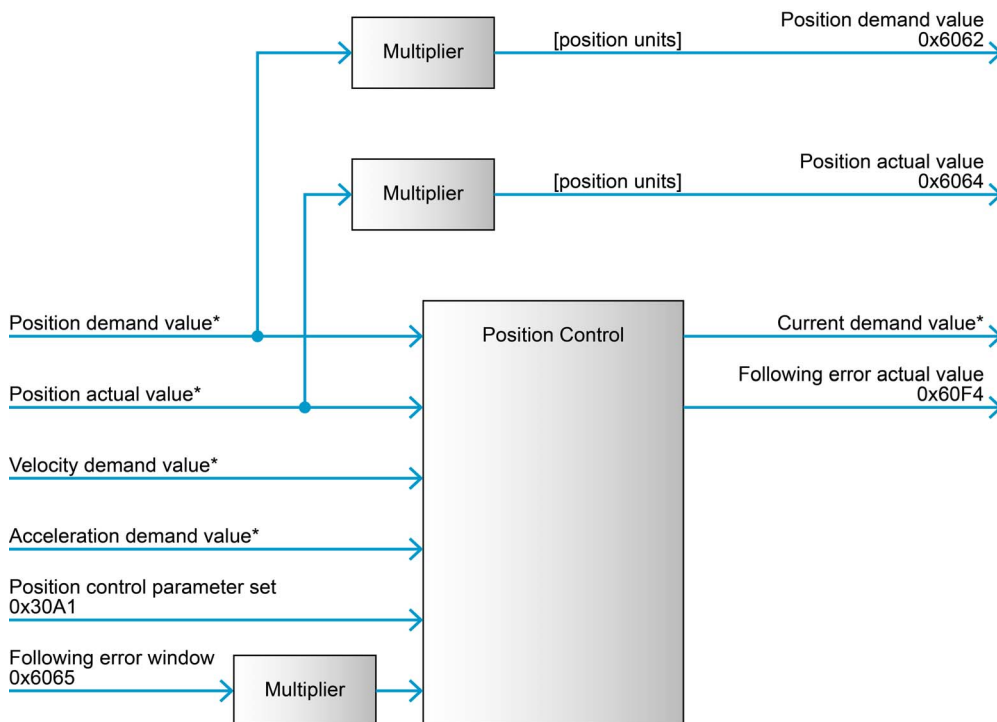
Figure 3-25 Position Control Function – Block diagram
