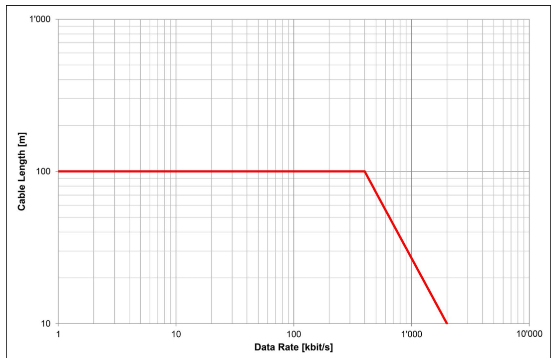
Figure 6-31 SSI encoder – Data rate vs. cable length
