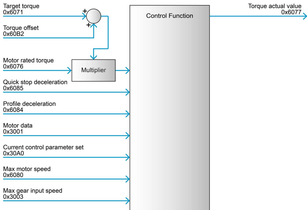
Figure 3-24 Cyclic Synchronous Torque Mode – Block diagram
