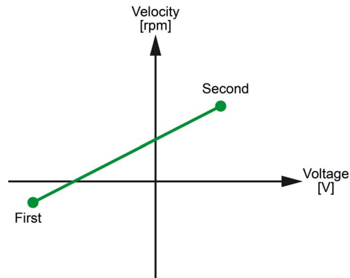
Figure 6-41 Analog input velocity set value properties – Set value
