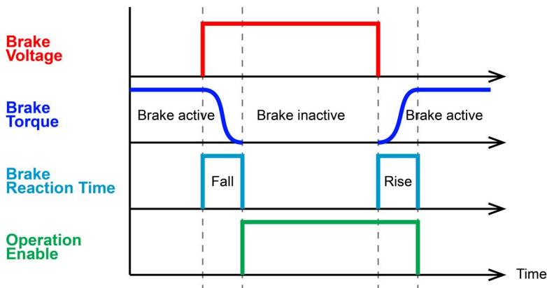
Figure 6-37 Holding brake activation timing (digital output polarity “High active”)
