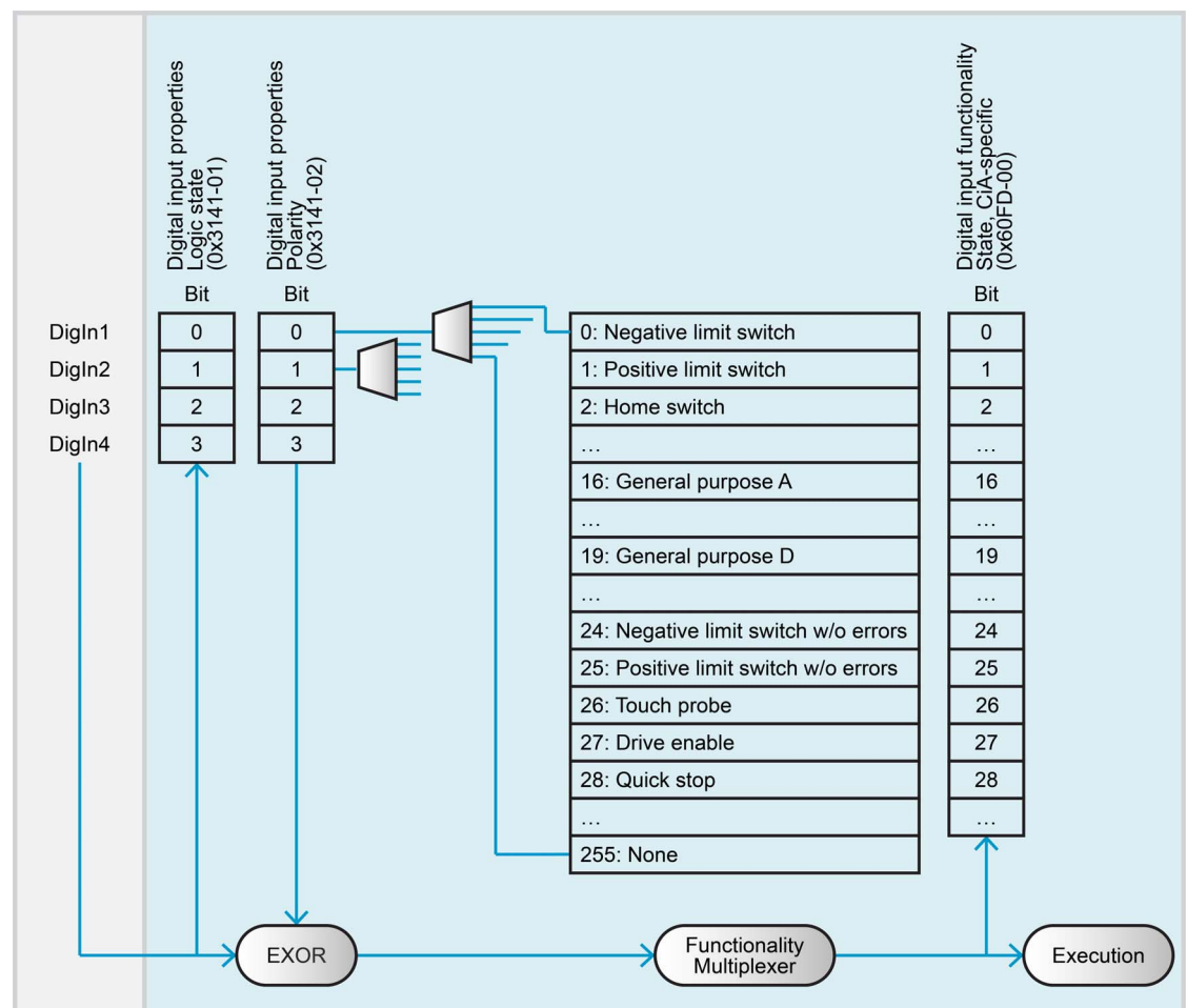
Figure 4-28 Digital input functionality
