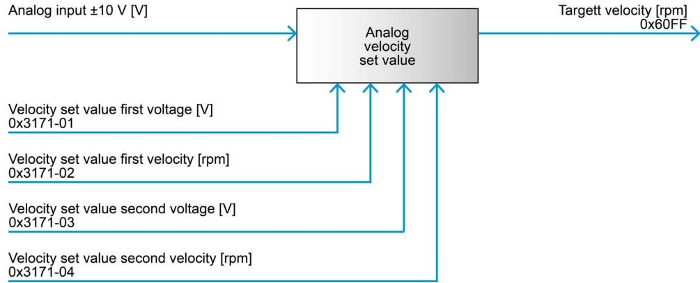
Figure 6-40 Analog input velocity set value properties – Setpoint function
