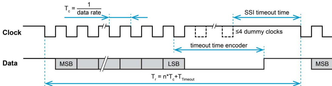
Figure 6-33 SSI encoder – Timing
