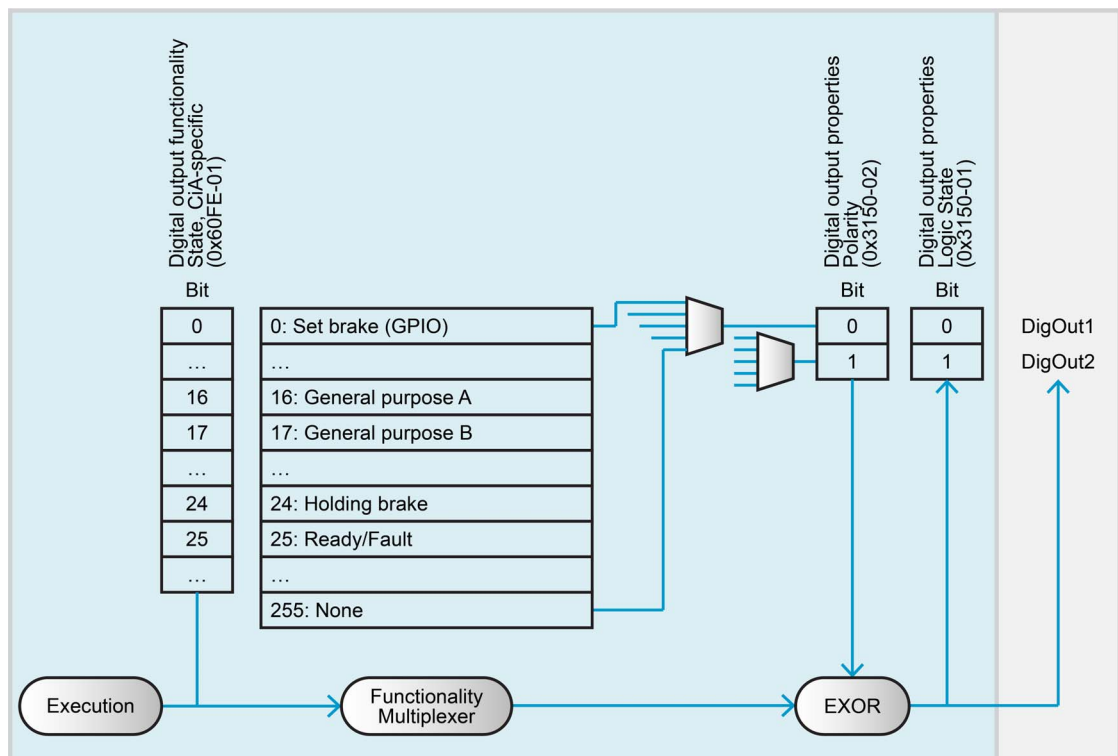
Figure 4-29 Digital output functionality
