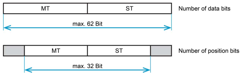
Figure 6-35 SSI encoder – Data bits
