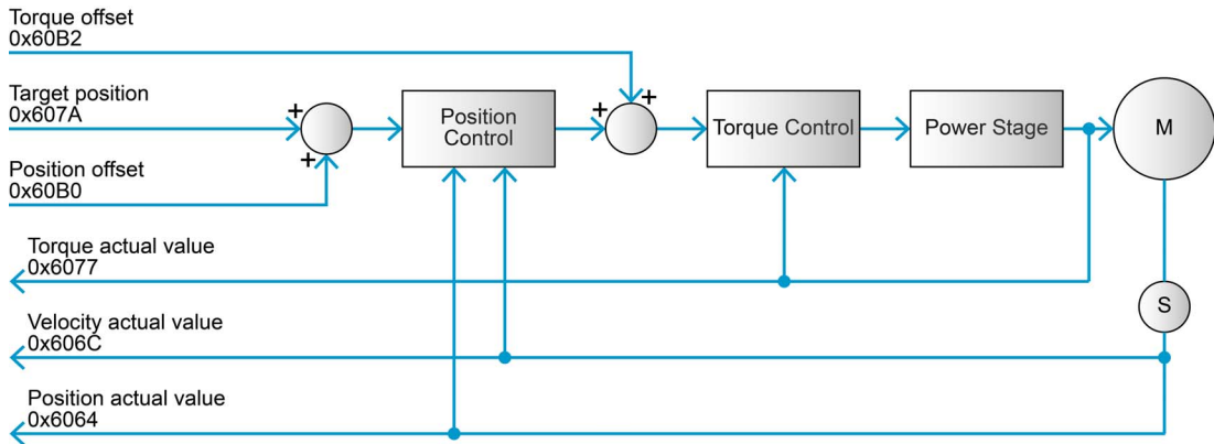
Figure 3-19 Cyclic Synchronous Position Mode – Overview
