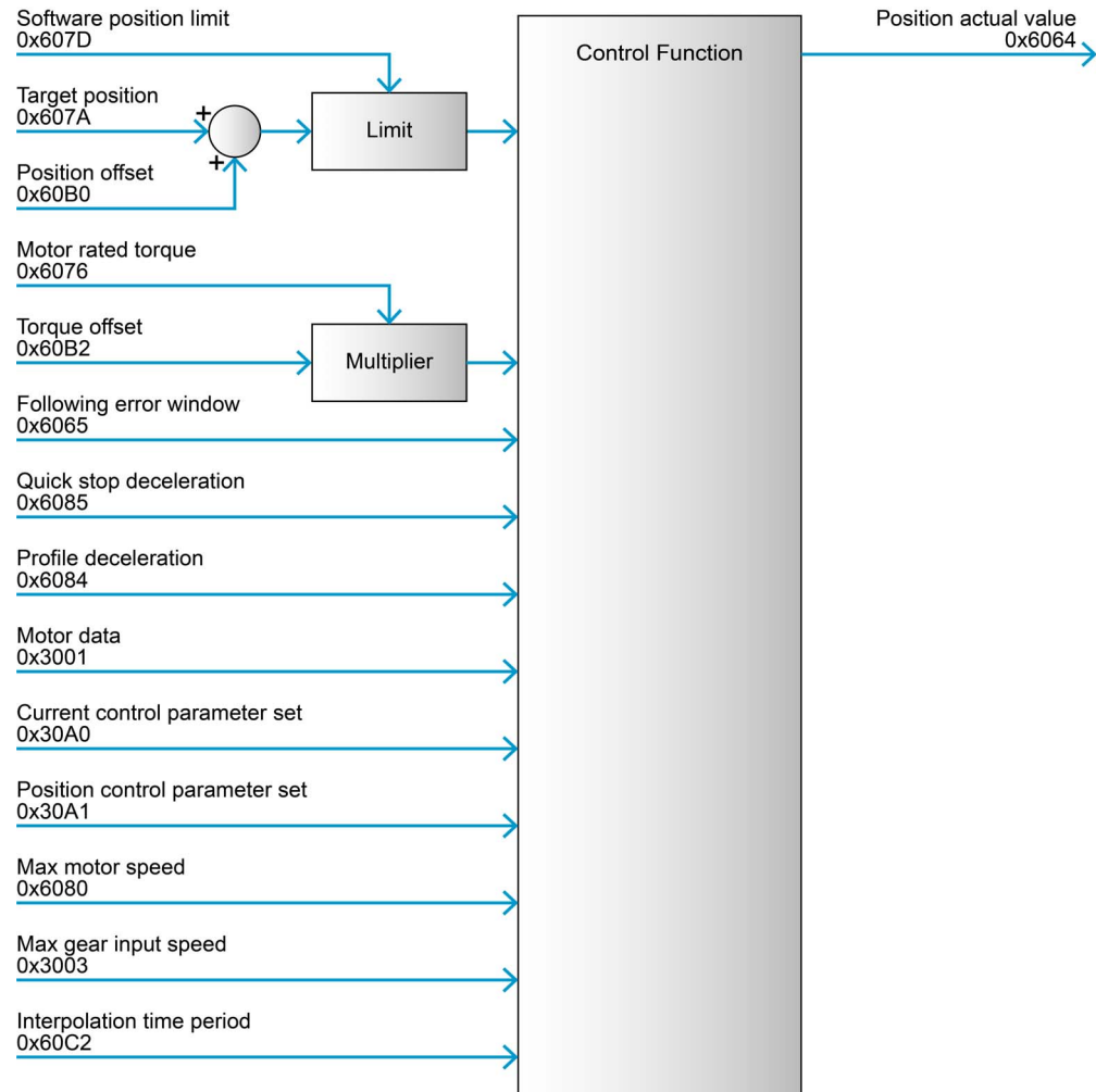
Figure 3-20 Cyclic Synchronous Position Mode – Block diagram
