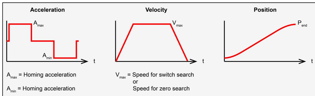
Figure 3-11 Homing trajectory – Linear ramp (trapezoidal profile)
