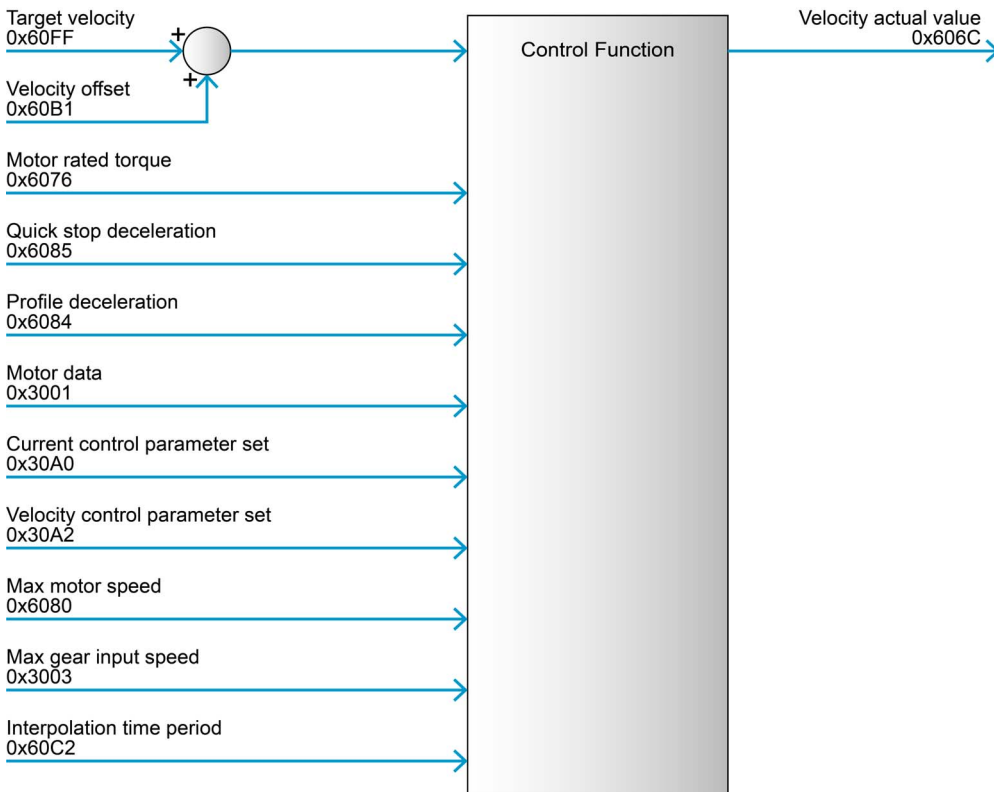
Figure 3-22 Cyclic Synchronous Velocity Mode – Block diagram
