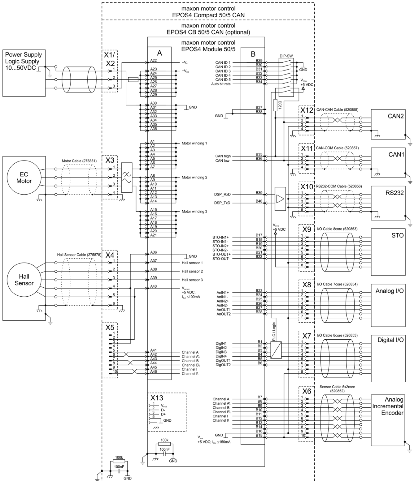
Figure 5-62 EC motor (Hall sensors & analog incremental encoder)
