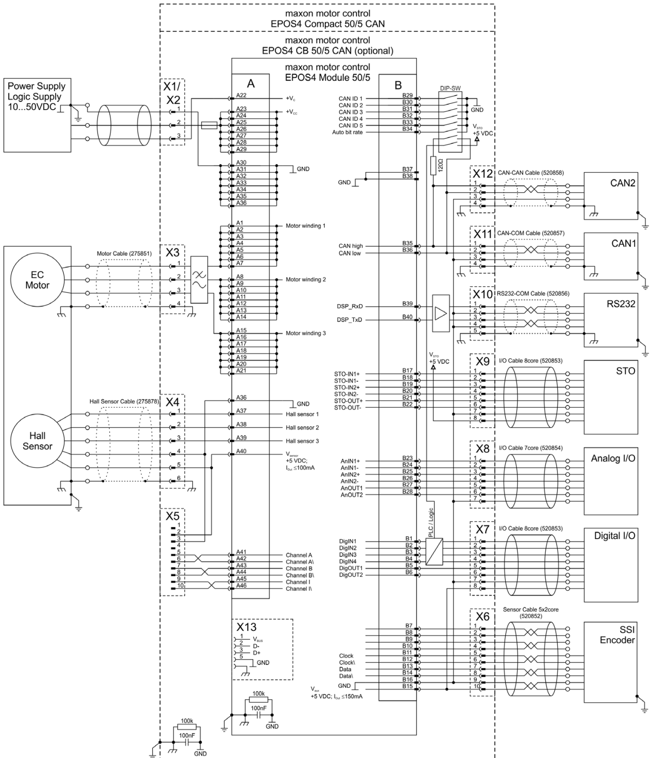
Figure 5-63 EC motor (Hall sensors & SSI encoder)
