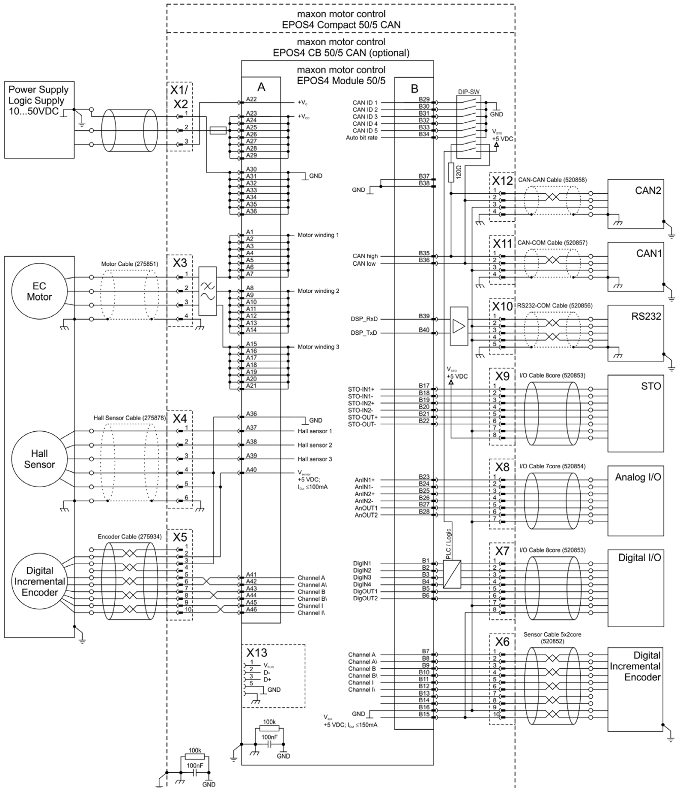
Figure 5-64 EC motor (Hall sensors & digital & digital incremental encoder)
