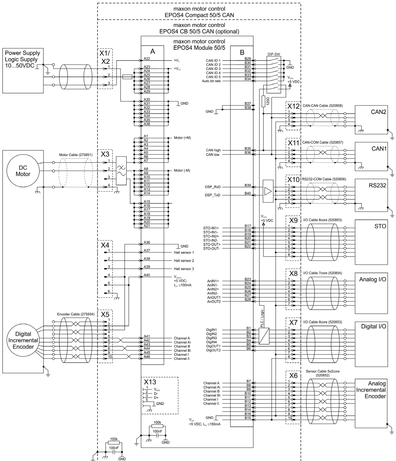
Figure 5-56 DC motor (digital & analog incremental encoder)
