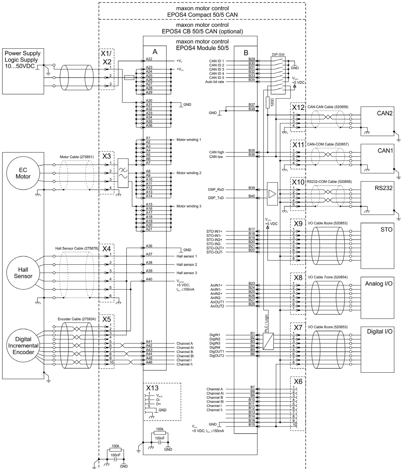
Figure 5-61 EC motor (Hall sensors & digital incremental encoder)
