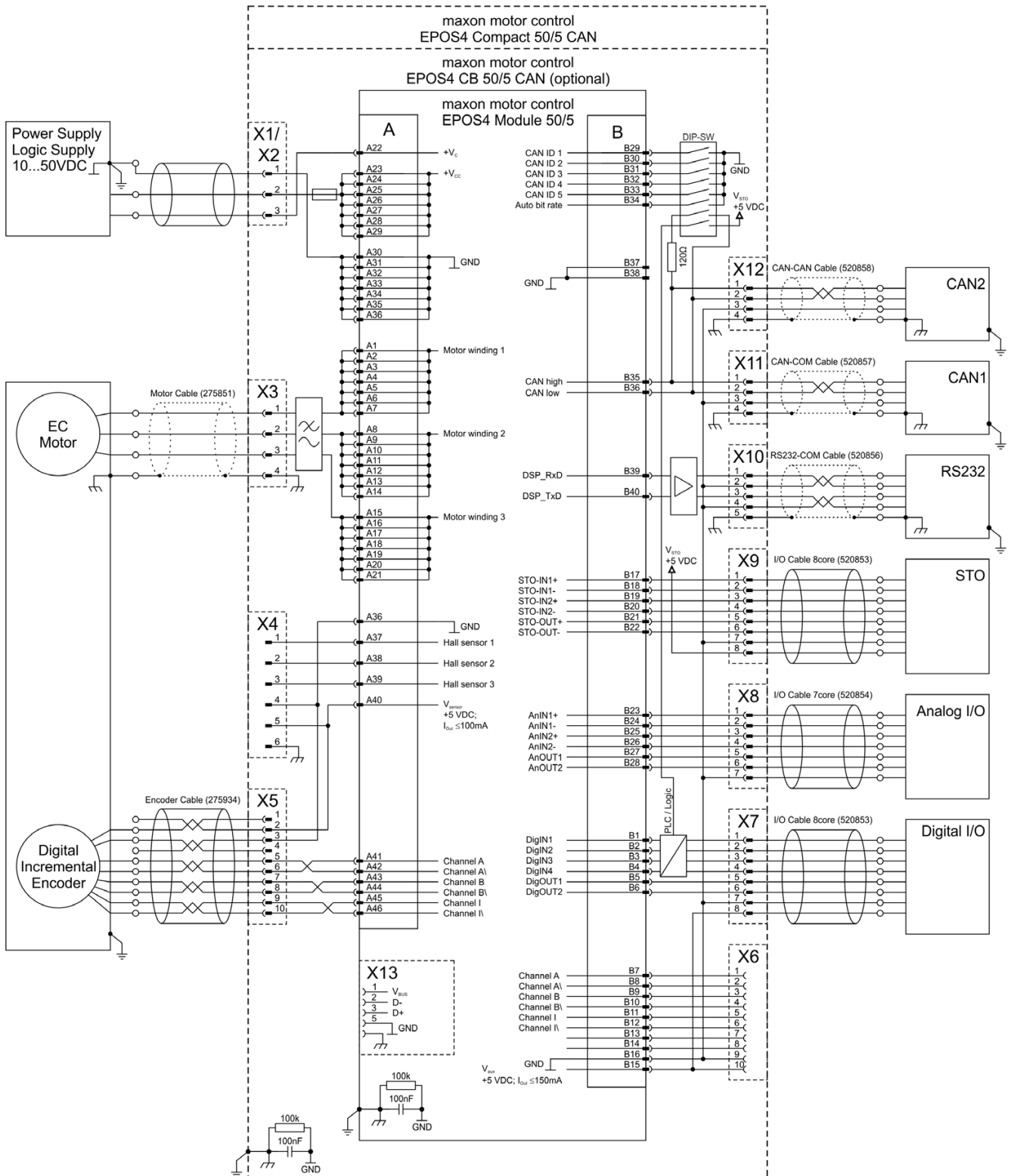
Figure 5-67 EC motor (digital incremental encoder)
