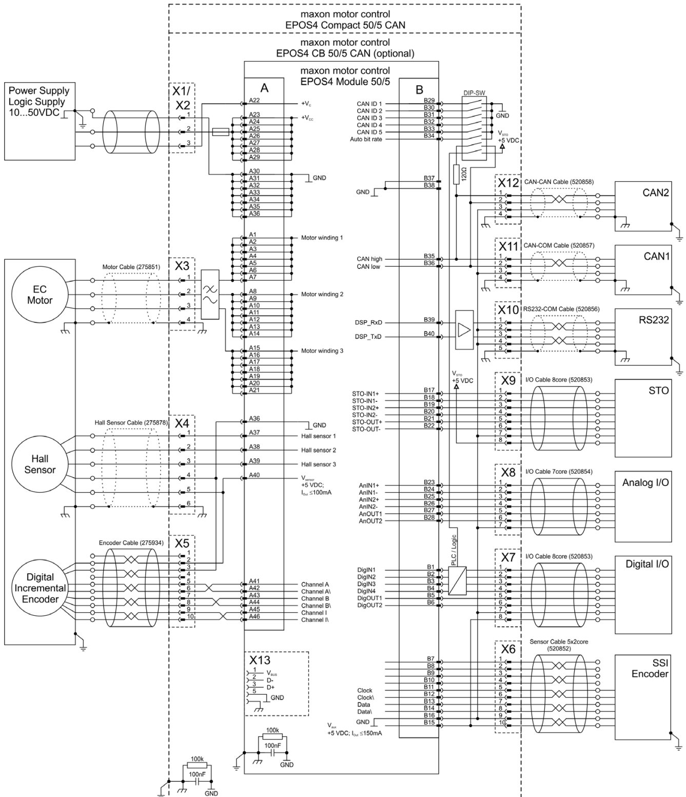
Figure 5-66 EC motor (Hall sensors & digital incremental & SSI encoder)
