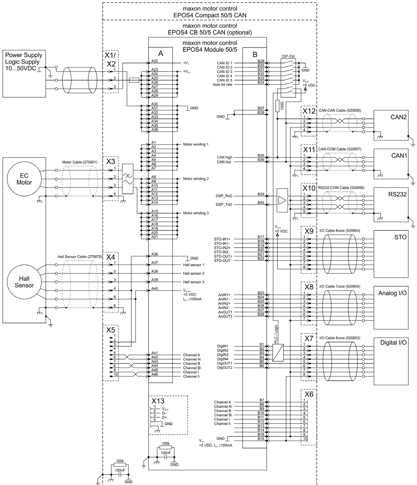
Figure 5-60 EC motor (Hall sensors)
