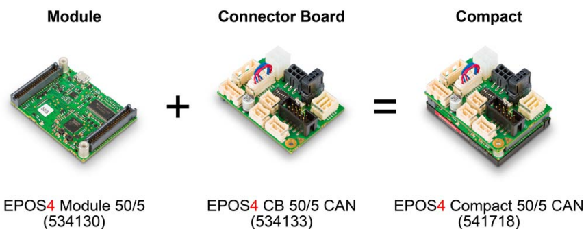
Figure 1-2 Configuration overview
