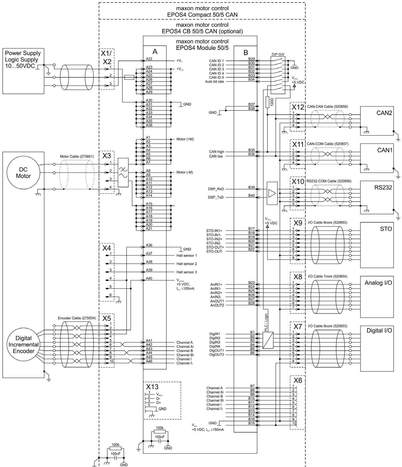
Figure 5-54 DC motor (digital incremental encoder)
