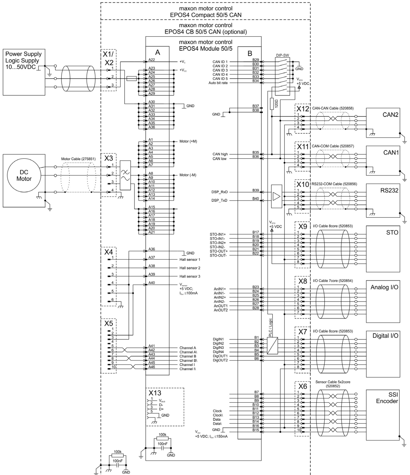
Figure 5-59 DC motor (SSI encoder)
