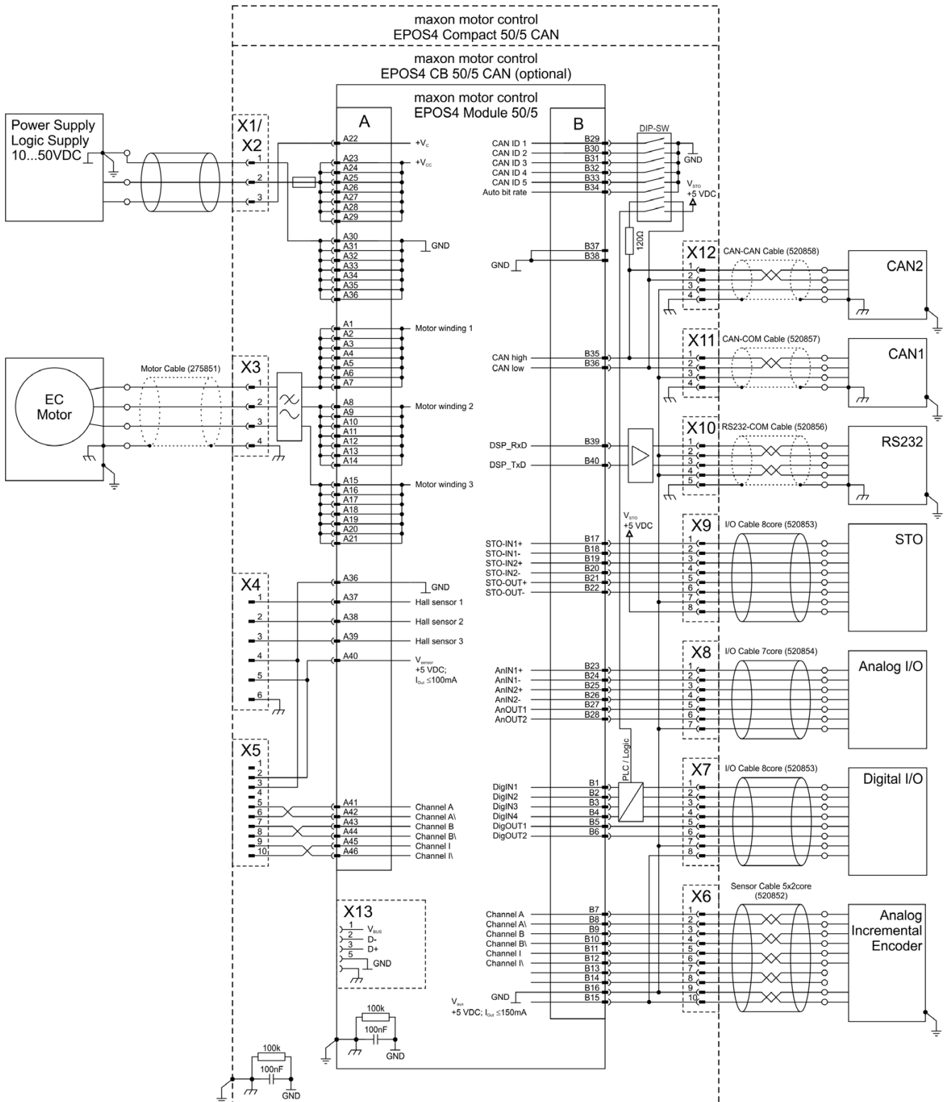
Figure 5-71 EC motor (analog incremental encoder)
