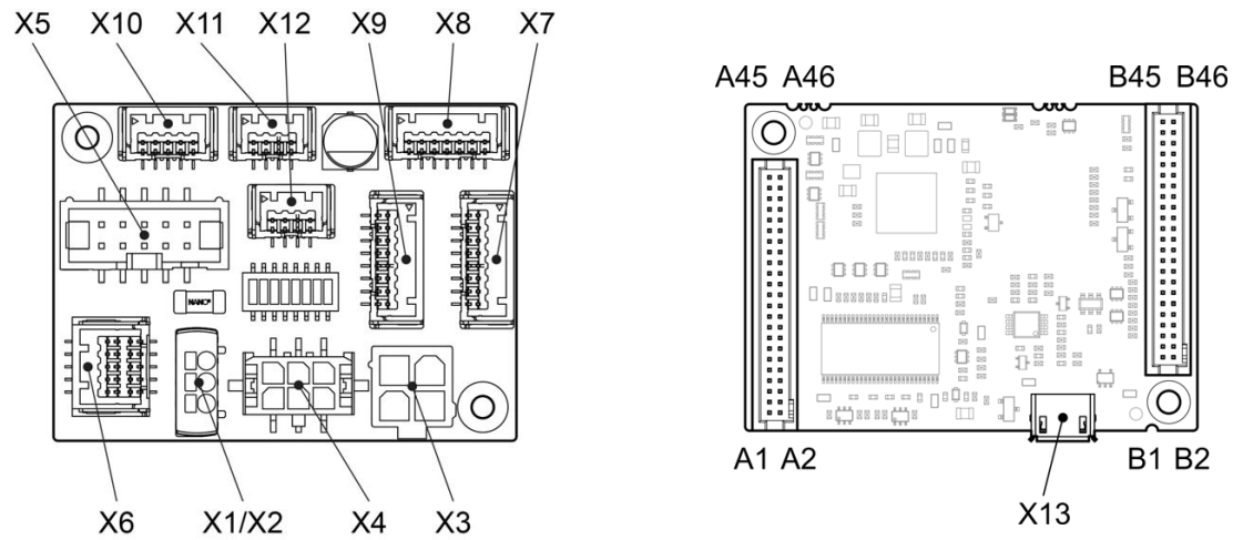
Figure 5-52 Interfaces – Designations and location
