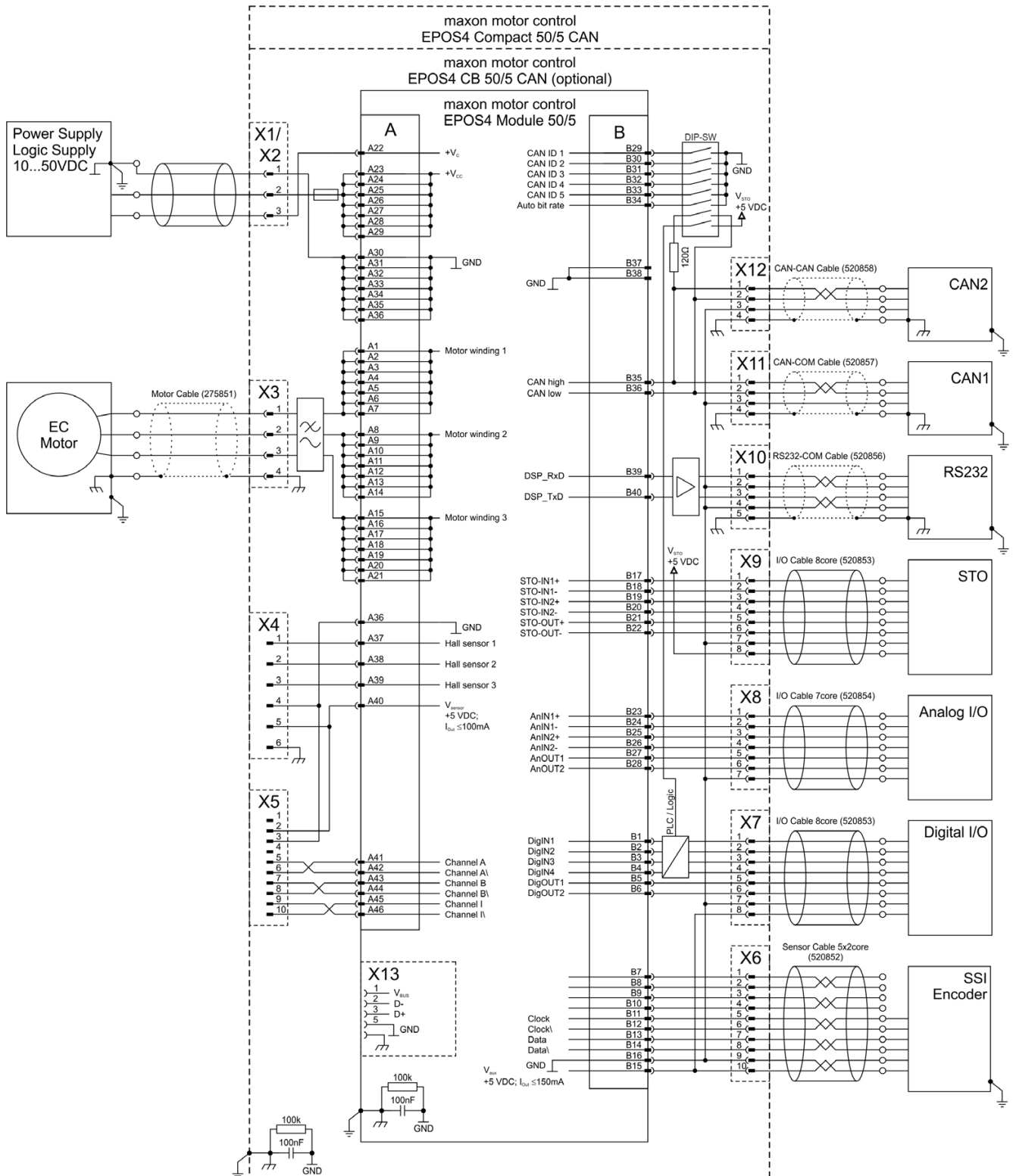
Figure 5-72 EC motor (SSI encoder)
