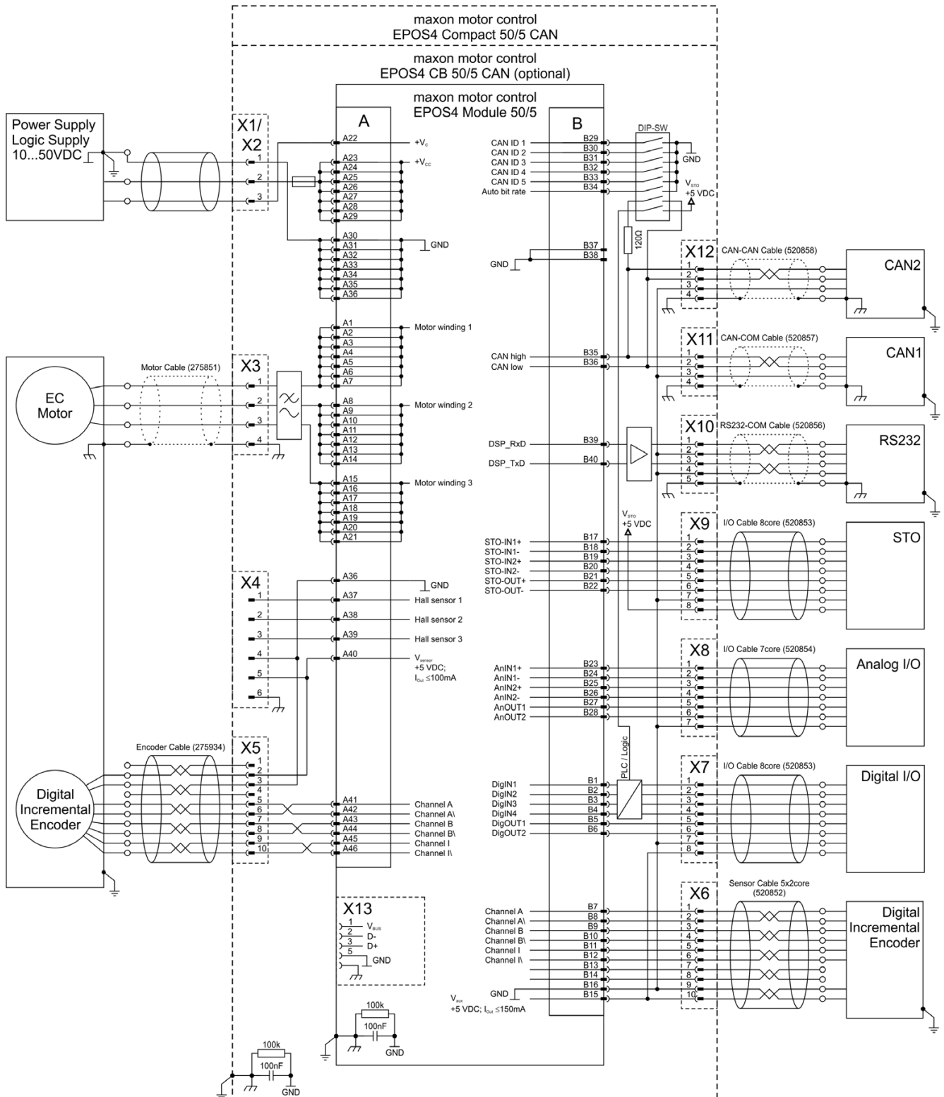
Figure 5-68 EC motor (digital & digital incremental encoder)
