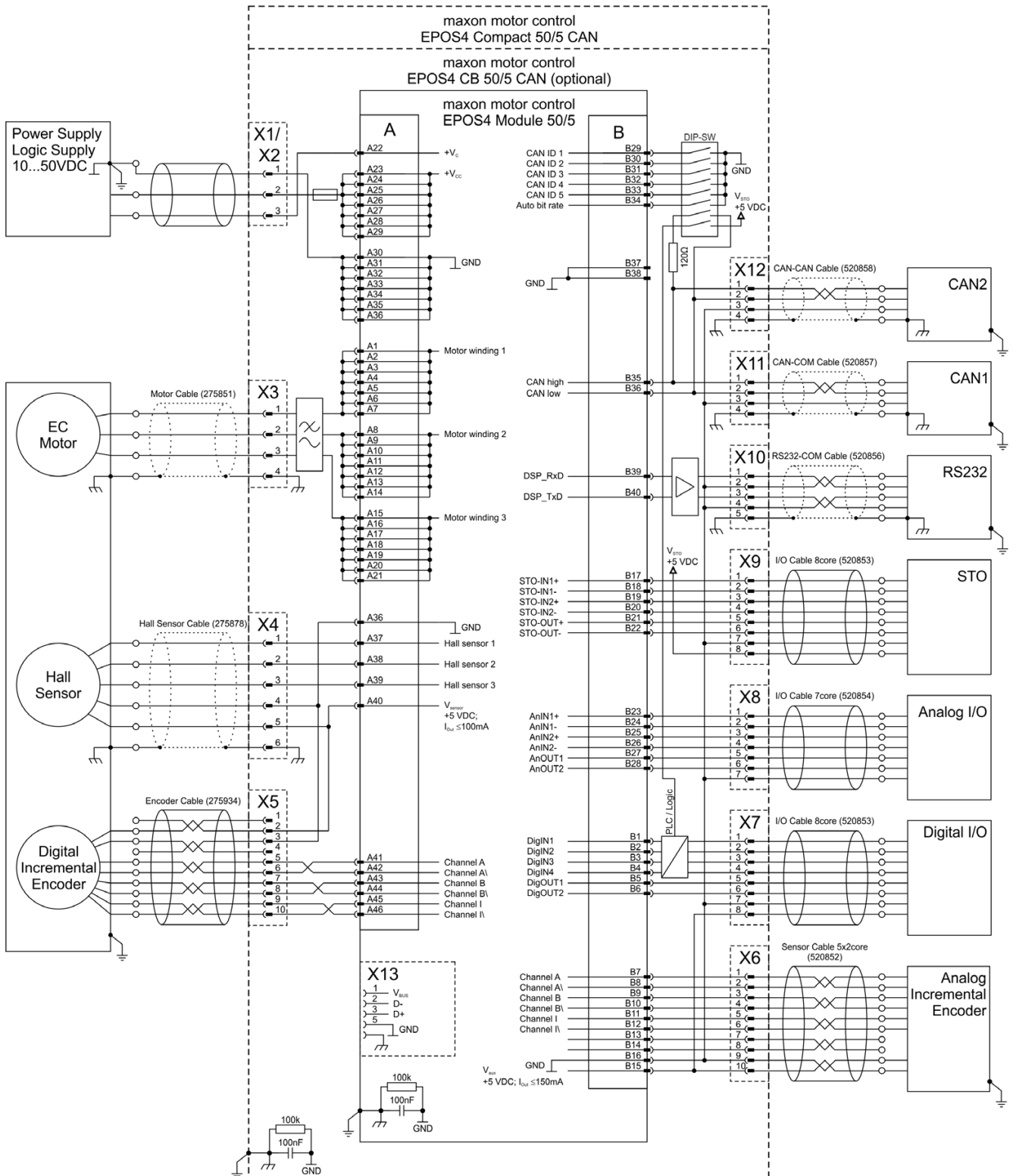
Figure 5-65 EC motor (Hall sensors &amp; digital &amp; analog incremental encoder)
