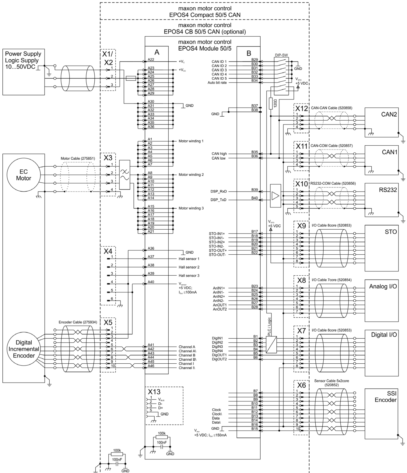
Figure 5-70 EC motor (digital & SSI encoder)
