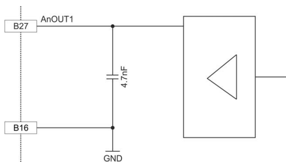
Figure 3-45 AnOUT1 circuit (analogously valid for AnOUT2)
