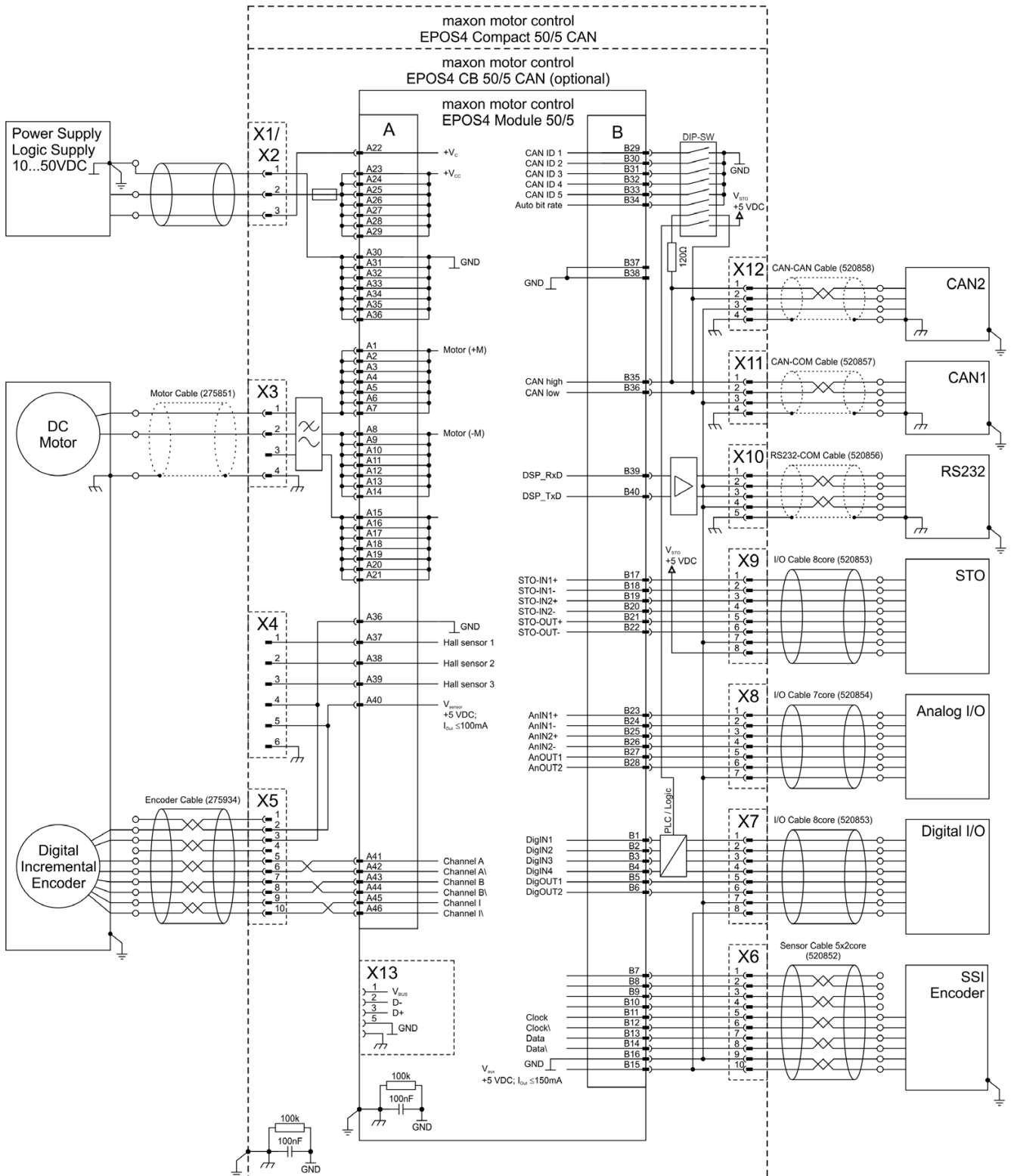
Figure 5-57 DC motor (digital incremental & SSI encoder)
