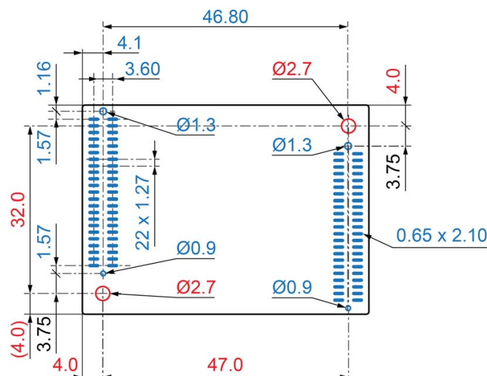
Figure 4-51 SMT footprint [mm] – Top View
