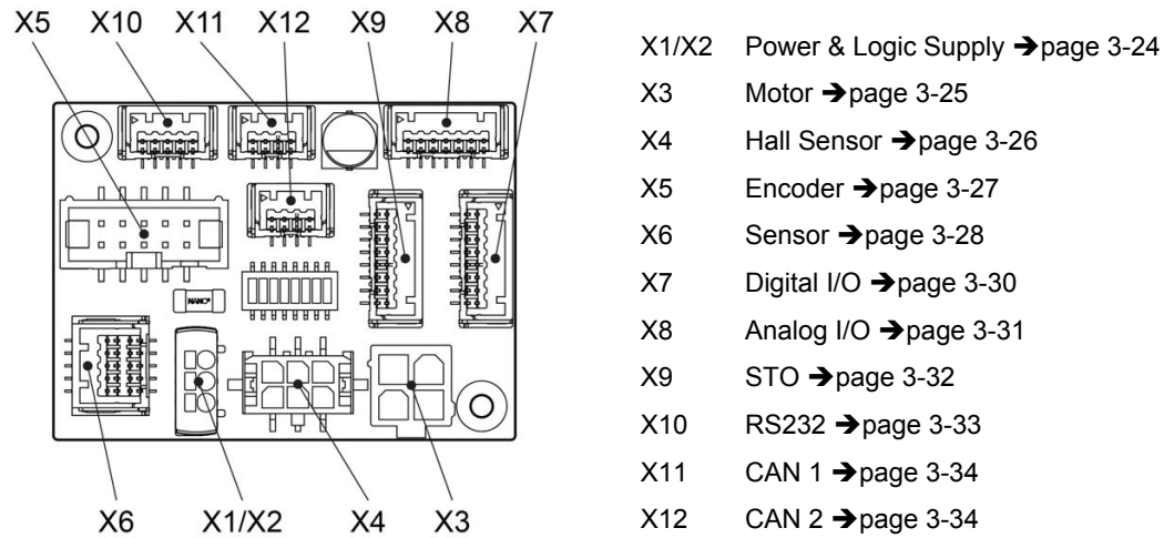
Figure 3-10 EPOS4 CB 50/5 CAN – Connectors
