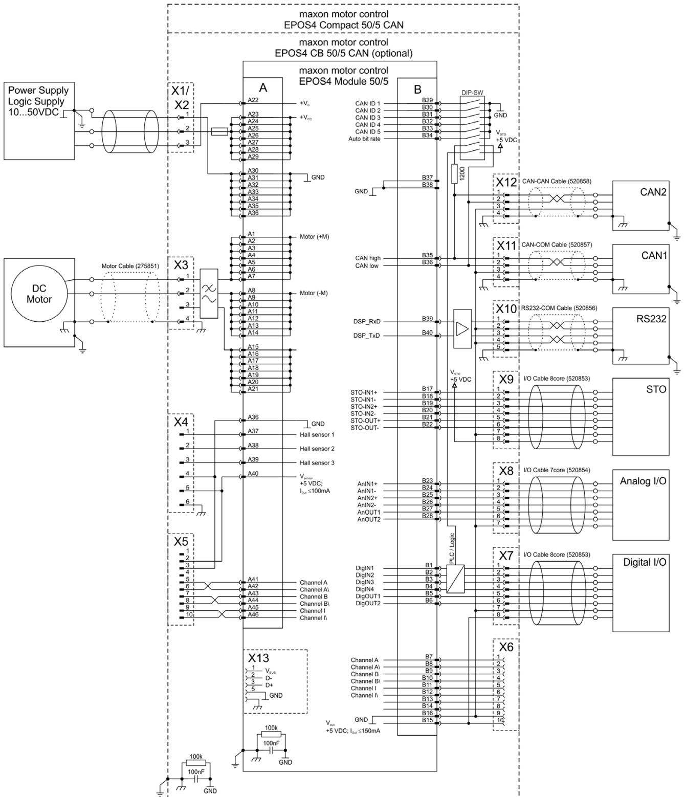
Figure 5-53 DC motor (no sensor)
