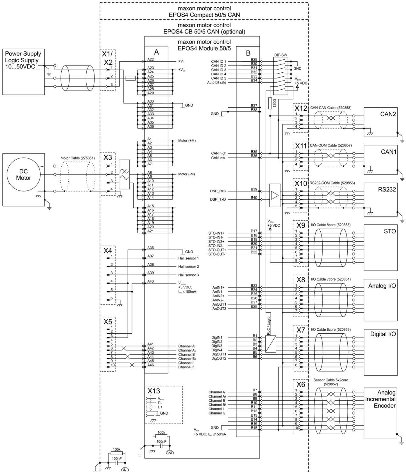
Figure 5-58 DC motor (analog incremental encoder)
