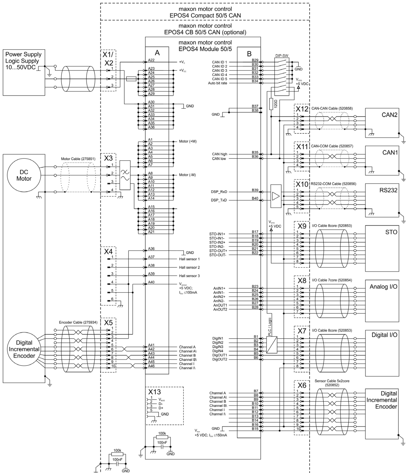
Figure 5-55 DC motor (digital & digital incremental encoder)
